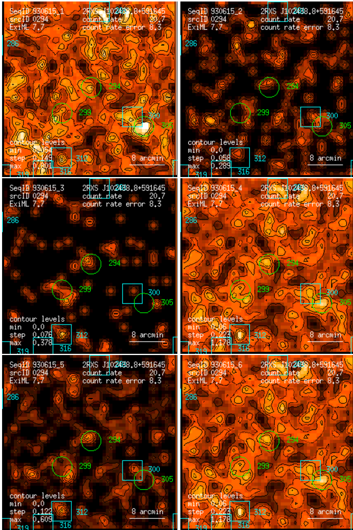
Figure 294: RASS 930615: detection 0294: band rate images, Gaussian filter: (1) PSPC channels 11 – 41, (2) 52 – 90, (3) 91 – 201, (4) 11 – 235, (5) 52 – 201, (6) 11 – 201. Broad band rates in counts/ks. Band rate contour levels in counts/ks/arcmin 2 .
