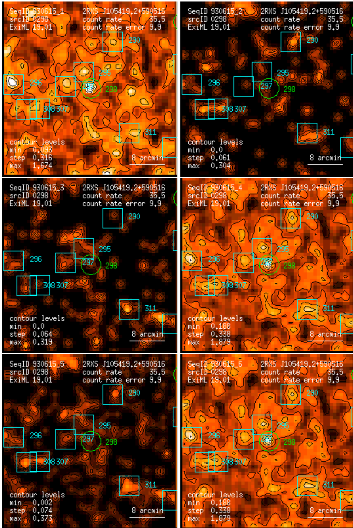
Figure 298: RASS 930615: detection 0298: band rate images, Gaussian filter: (1) PSPC channels 11 – 41, (2) 52 – 90, (3) 91 – 201, (4) 11 – 235, (5) 52 – 201, (6) 11 – 201. Broad band rates in counts/ks. Band rate contour levels in counts/ks/arcmin 2 .
