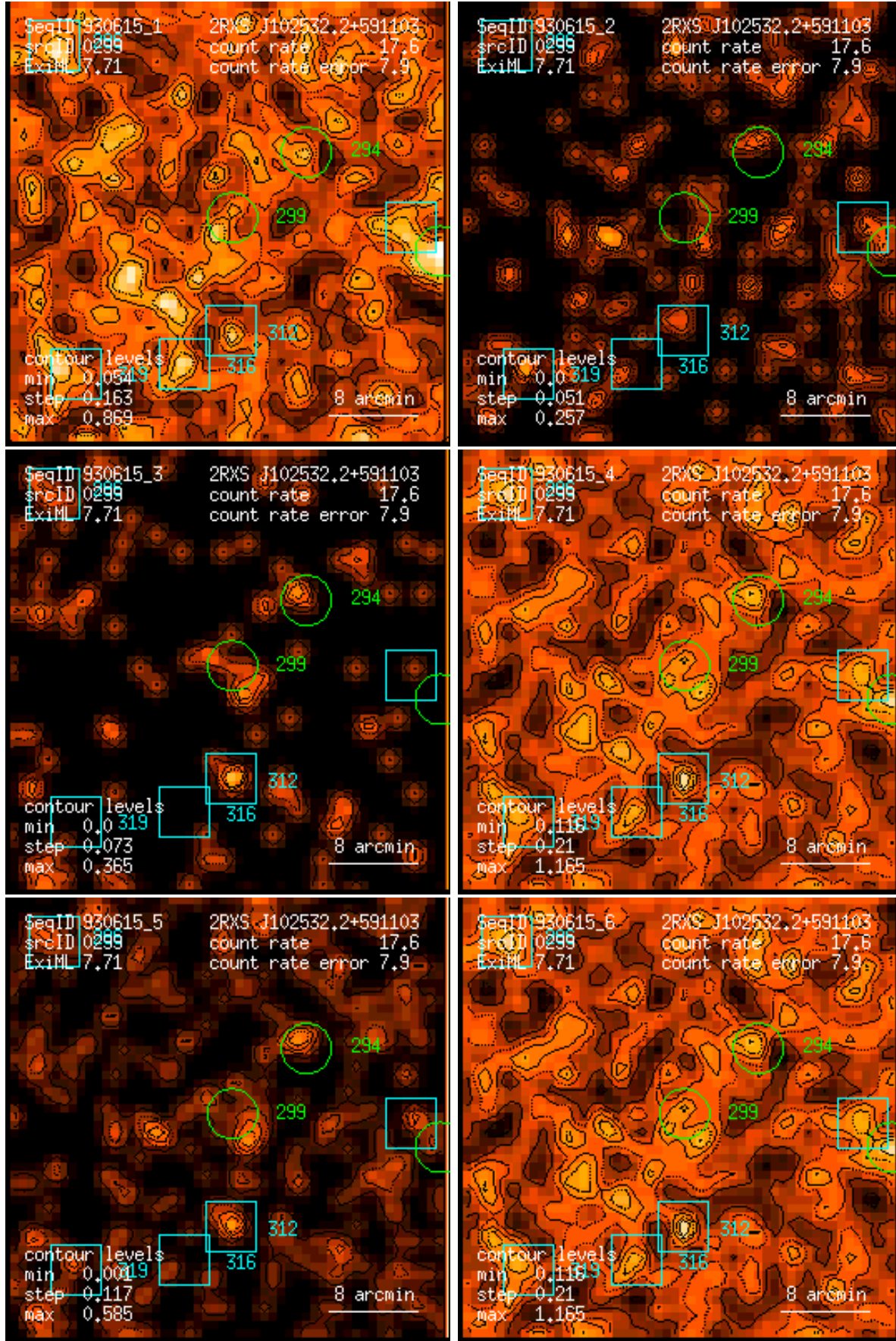
Figure 299: RASS 930615: detection 0299: band rate images, Gaussian filter: (1) PSPC channels 11 – 41, (2) 52 – 90, (3) 91 – 201, (4) 11 – 235, (5) 52 – 201, (6) 11 – 201. Broad band rates in counts/ks. Band rate contour levels in counts/ks/arcmin 2 .
