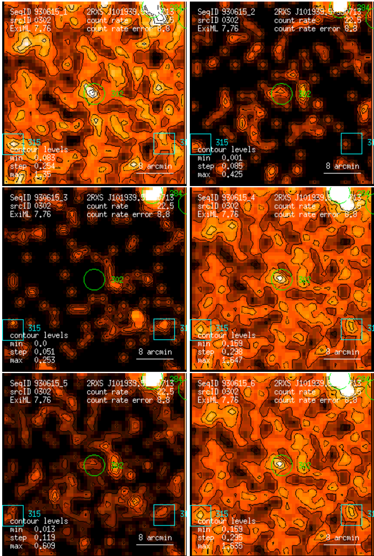
Figure 302: RASS 930615: detection 0302: band rate images, Gaussian filter: (1) PSPC channels 11 – 41, (2) 52 – 90, (3) 91 – 201, (4) 11 – 235, (5) 52 – 201, (6) 11 – 201. Broad band rates in counts/ks. Band rate contour levels in counts/ks/arcmin 2 .
