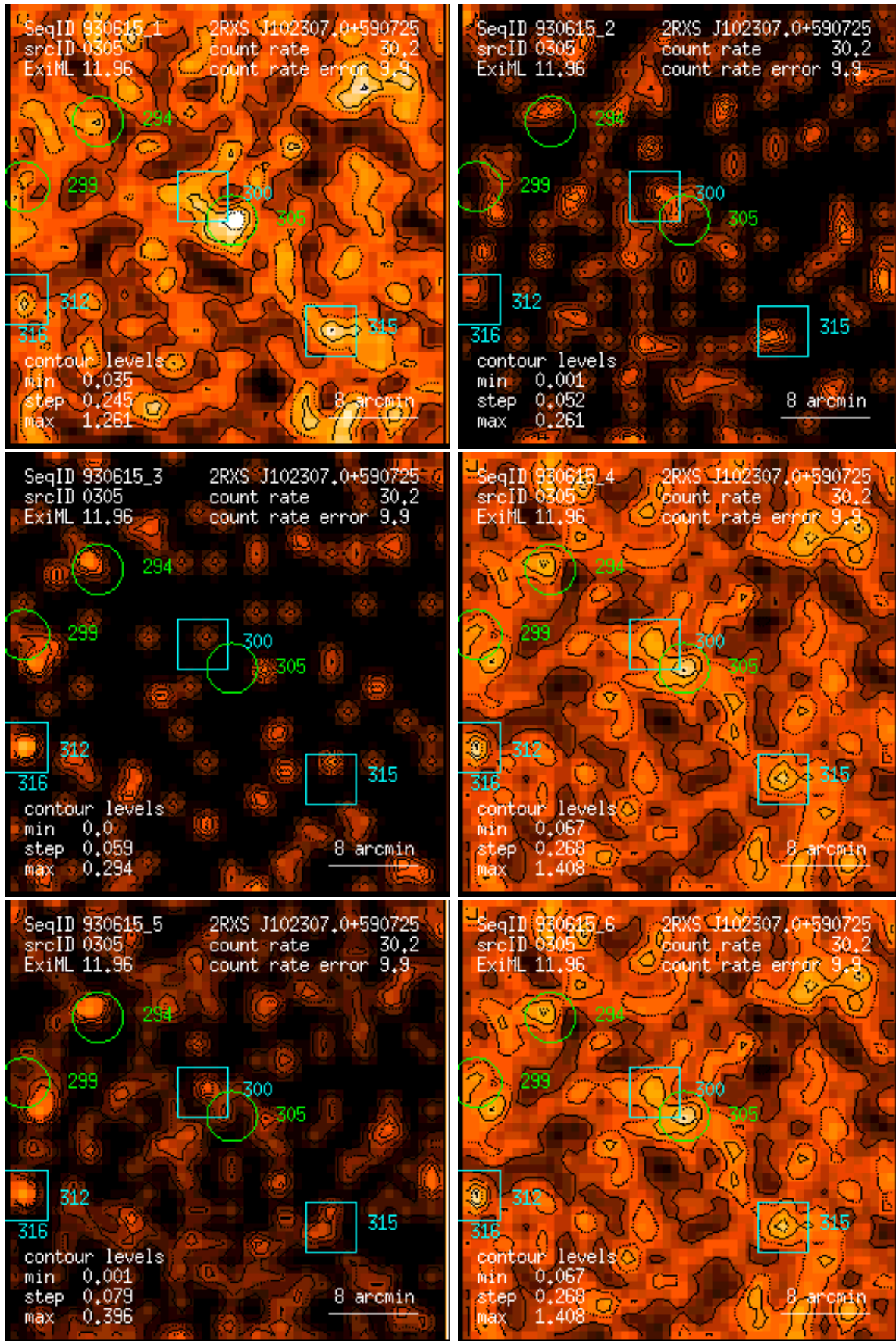
Figure 305: RASS 930615: detection 0305: band rate images, Gaussian filter: (1) PSPC channels 11 – 41, (2) 52 – 90, (3) 91 – 201, (4) 11 – 235, (5) 52 – 201, (6) 11 – 201. Broad band rates in counts/ks. Band rate contour levels in counts/ks/arcmin 2 .
