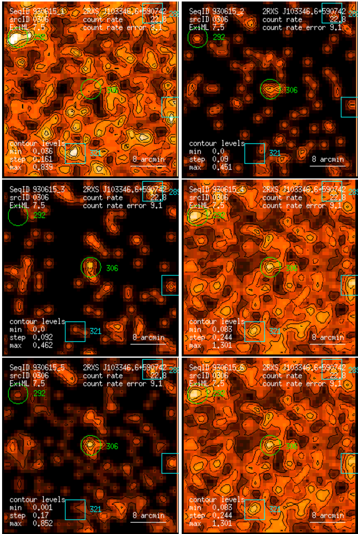
Figure 306: RASS 930615: detection 0306: band rate images, Gaussian filter: (1) PSPC channels 11 – 41, (2) 52 – 90, (3) 91 – 201, (4) 11 – 235, (5) 52 – 201, (6) 11 – 201. Broad band rates in counts/ks. Band rate contour levels in counts/ks/arcmin 2 .
