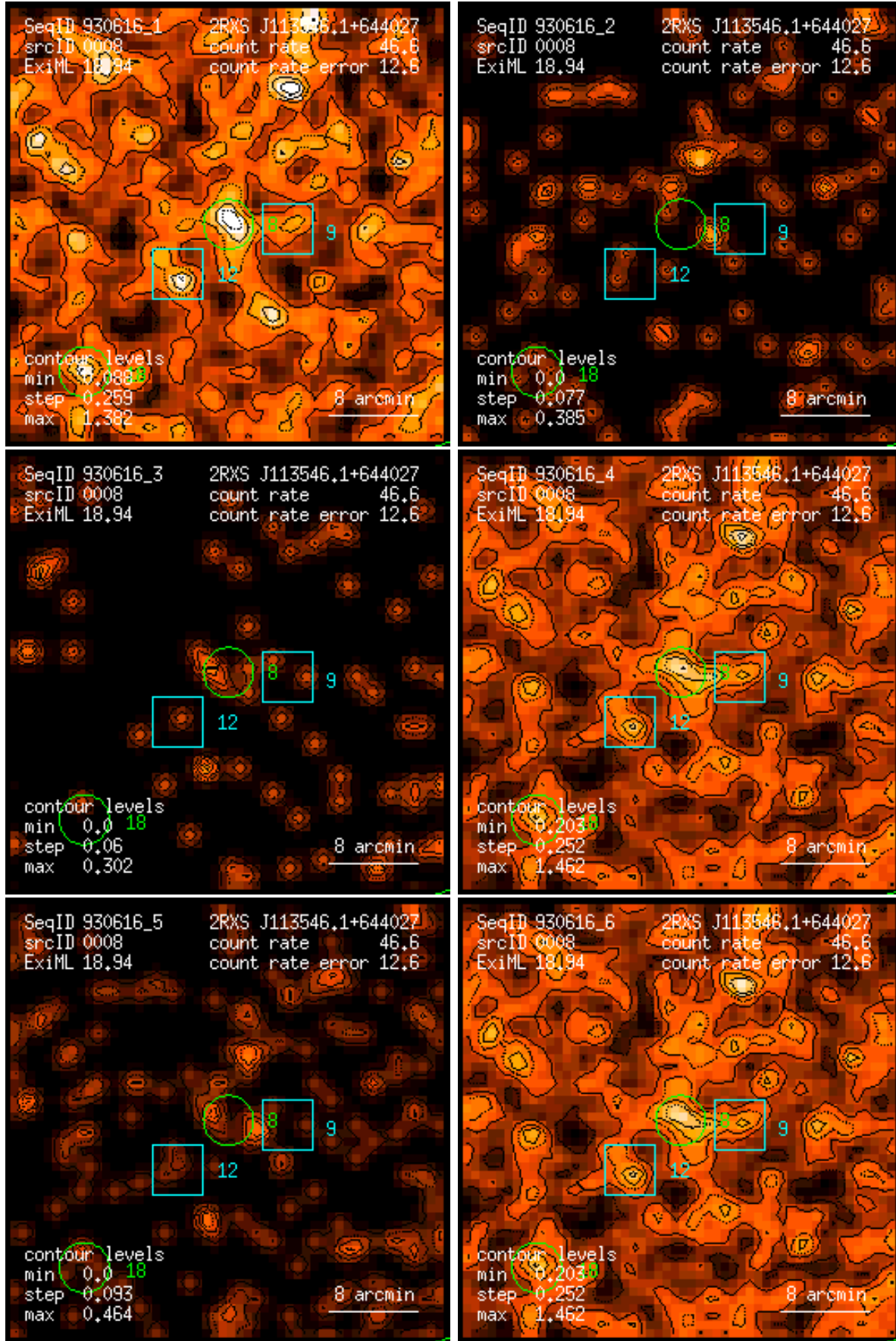
Figure 8: RASS 930616: detection 0008: band rate images, Gaussian filter: (1) PSPC channels 11 – 41, (2) 52 – 90, (3) 91 – 201, (4) 11 – 235, (5) 52 – 201, (6) 11 – 201. Broad band rates in counts/ks. Band rate contour levels in counts/ks/arcmin 2 .
