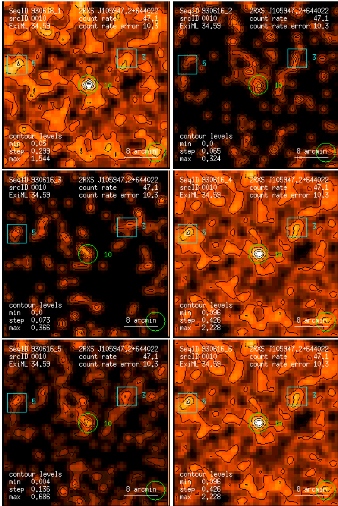
Figure 10: RASS 930616: detection 0010: band rate images, Gaussian filter: (1) PSPC channels 11 – 41, (2) 52 – 90, (3) 91 – 201, (4) 11 – 235, (5) 52 – 201, (6) 11 – 201. Broad band rates in counts/ks. Band rate contour levels in counts/ks/arcmin 2 .
