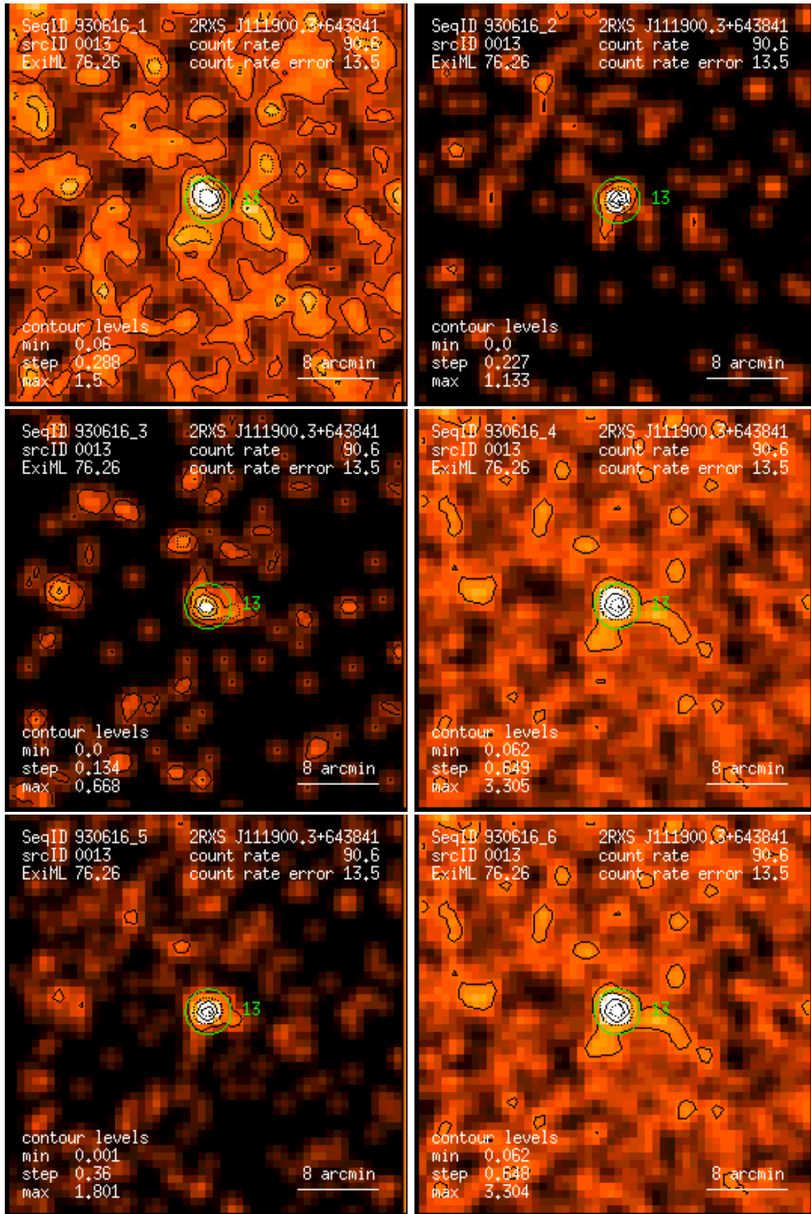
Figure 13: RASS 930616: detection 0013: band rate images, Gaussian filter: (1) PSPC channels 11 – 41, (2) 52 – 90, (3) 91 – 201, (4) 11 – 235, (5) 52 – 201, (6) 11 – 201. Broad band rates in counts/ks. Band rate contour levels in counts/ks/arcmin 2 .
