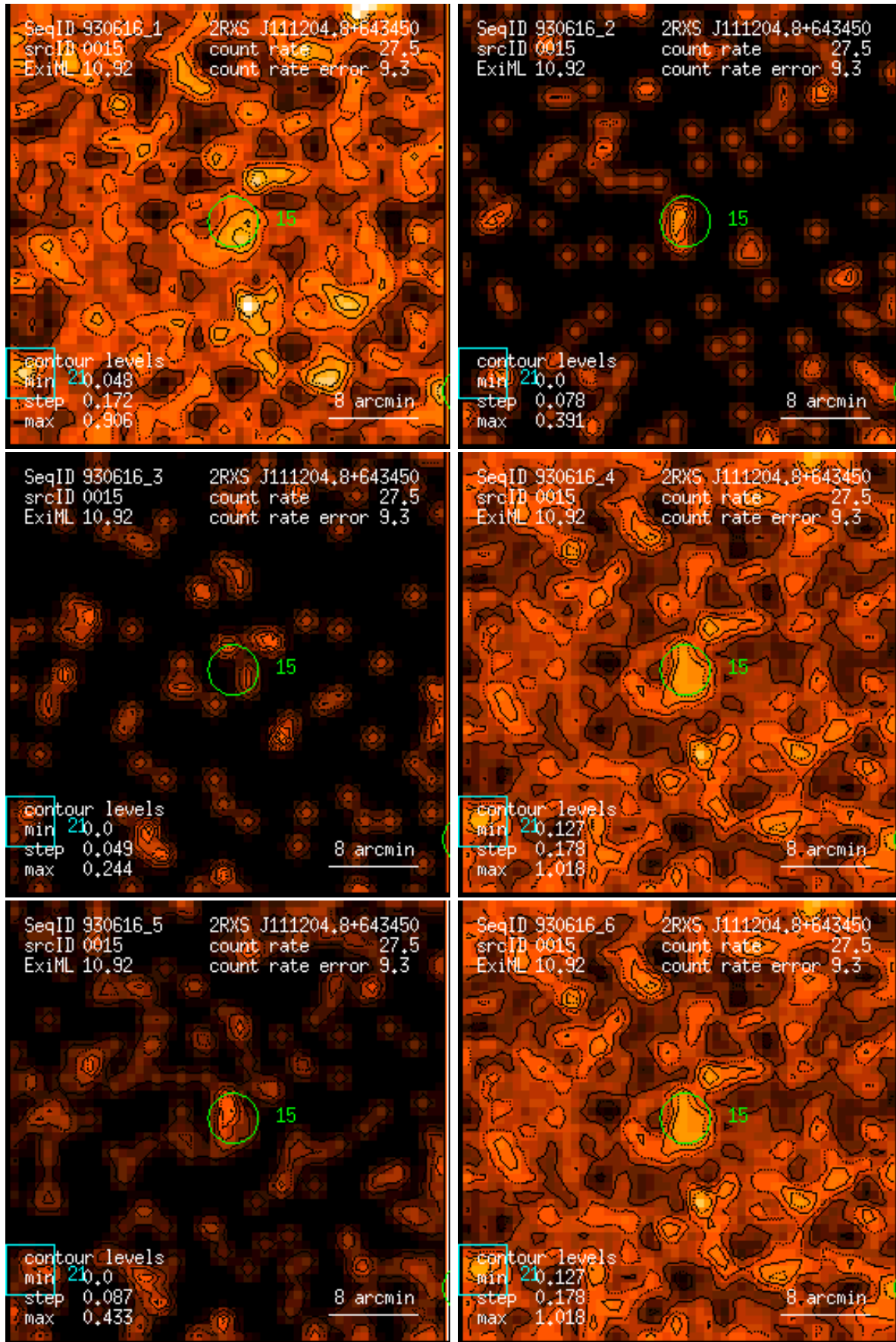
Figure 15: RASS 930616: detection 0015: band rate images, Gaussian filter: (1) PSPC channels 11 – 41, (2) 52 – 90, (3) 91 – 201, (4) 11 – 235, (5) 52 – 201, (6) 11 – 201. Broad band rates in counts/ks. Band rate contour levels in counts/ks/arcmin 2 .
