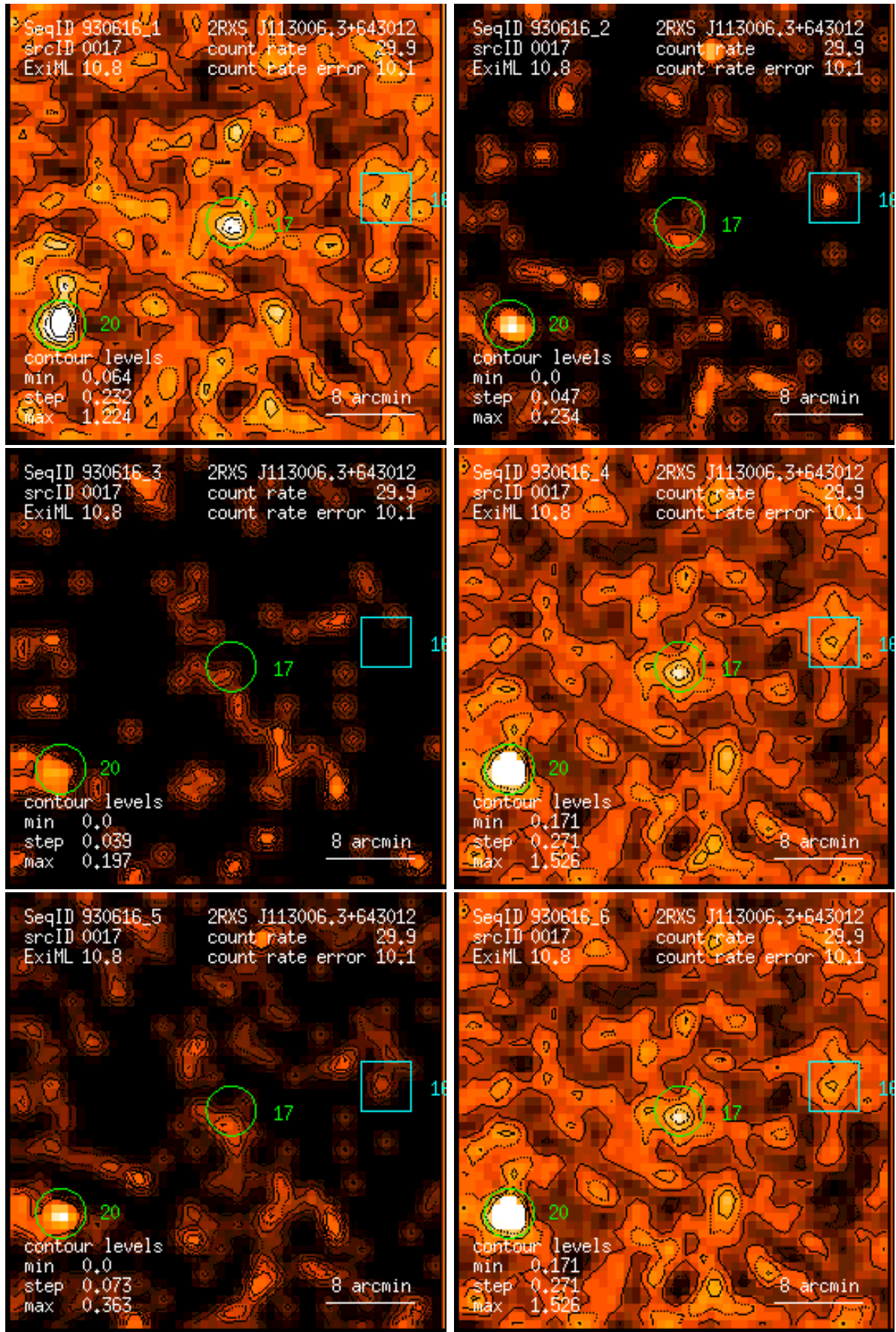
Figure 17: RASS 930616: detection 0017: band rate images, Gaussian filter: (1) PSPC channels 11 – 41, (2) 52 – 90, (3) 91 – 201, (4) 11 – 235, (5) 52 – 201, (6) 11 – 201. Broad band rates in counts/ks. Band rate contour levels in counts/ks/arcmin 2 .
