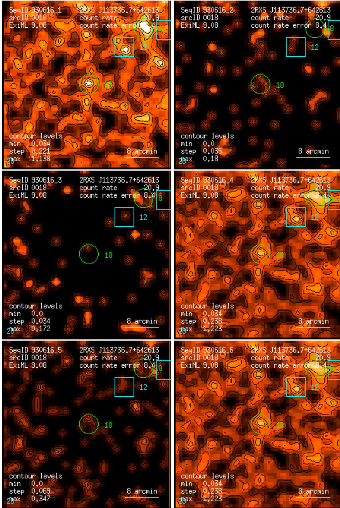
Figure 18: RASS 930616: detection 0018: band rate images, Gaussian filter: (1) PSPC channels 11 – 41, (2) 52 – 90, (3) 91 – 201, (4) 11 – 235, (5) 52 – 201, (6) 11 – 201. Broad band rates in counts/ks. Band rate contour levels in counts/ks/arcmin 2 .
