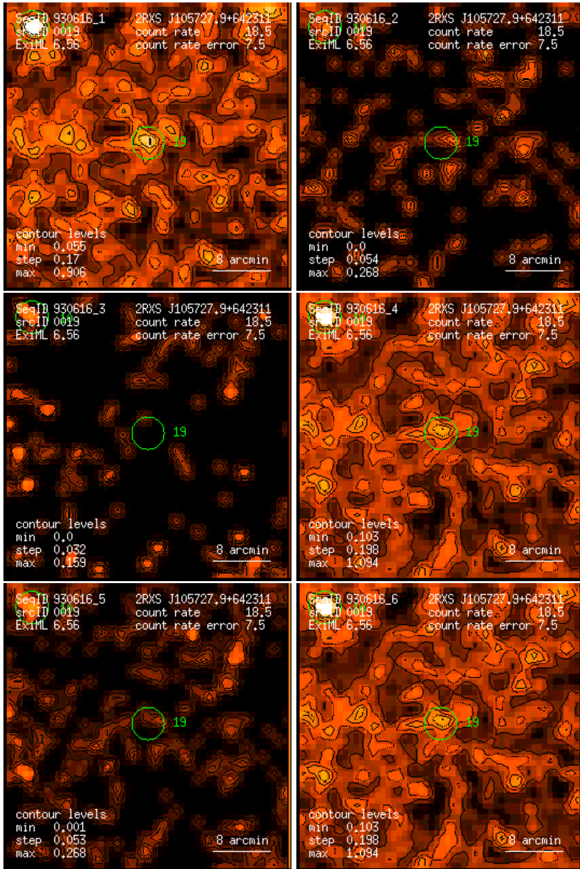
Figure 19: RASS 930616: detection 0019: band rate images, Gaussian filter: (1) PSPC channels 11 – 41, (2) 52 – 90, (3) 91 – 201, (4) 11 – 235, (5) 52 – 201, (6) 11 – 201. Broad band rates in counts/ks. Band rate contour levels in counts/ks/arcmin 2 .
