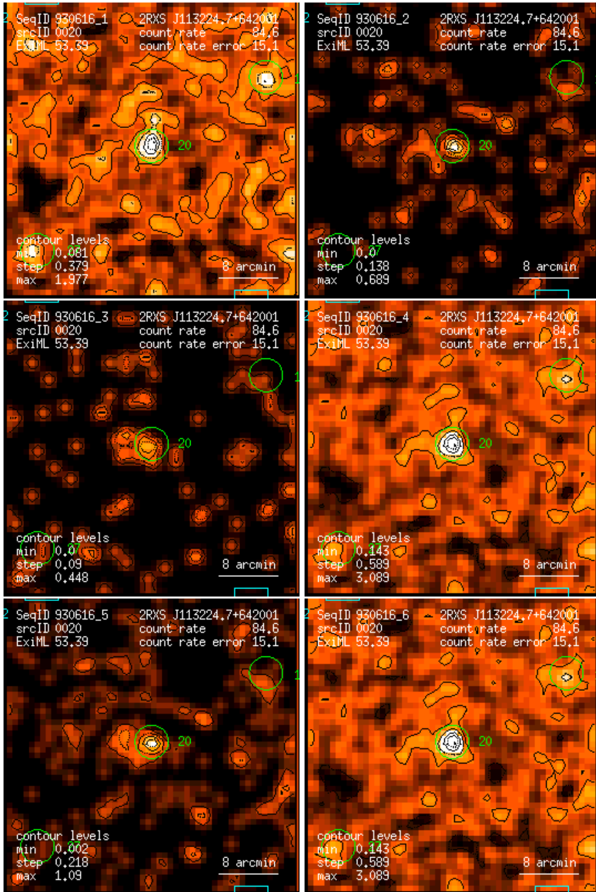
Figure 20: RASS 930616: detection 0020: band rate images, Gaussian filter: (1) PSPC channels 11 – 41, (2) 52 – 90, (3) 91 – 201, (4) 11 – 235, (5) 52 – 201, (6) 11 – 201. Broad band rates in counts/ks. Band rate contour levels in counts/ks/arcmin 2 .
