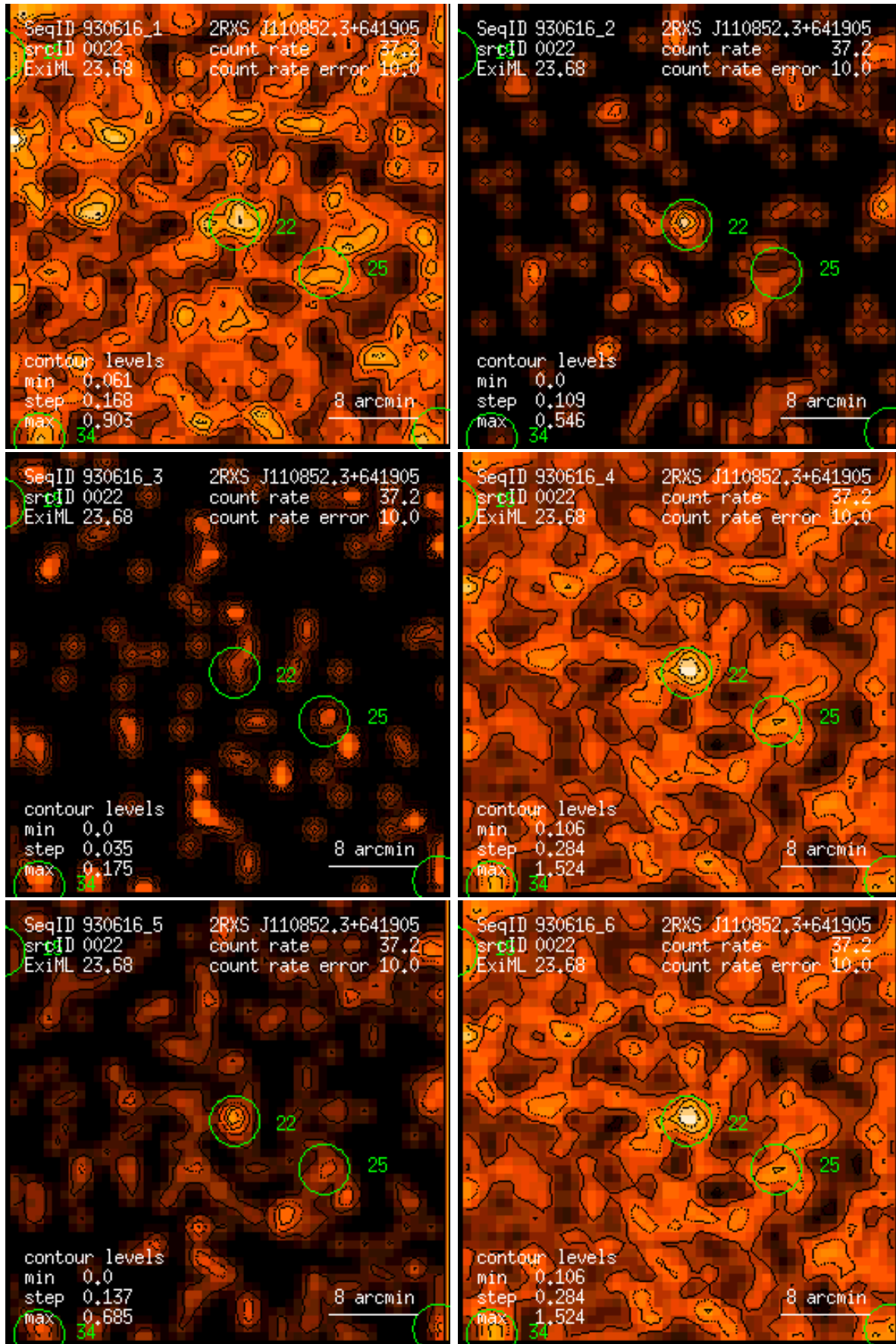
Figure 22: RASS 930616: detection 0022: band rate images, Gaussian filter: (1) PSPC channels 11 – 41, (2) 52 – 90, (3) 91 – 201, (4) 11 – 235, (5) 52 – 201, (6) 11 – 201. Broad band rates in counts/ks. Band rate contour levels in counts/ks/arcmin 2 .
