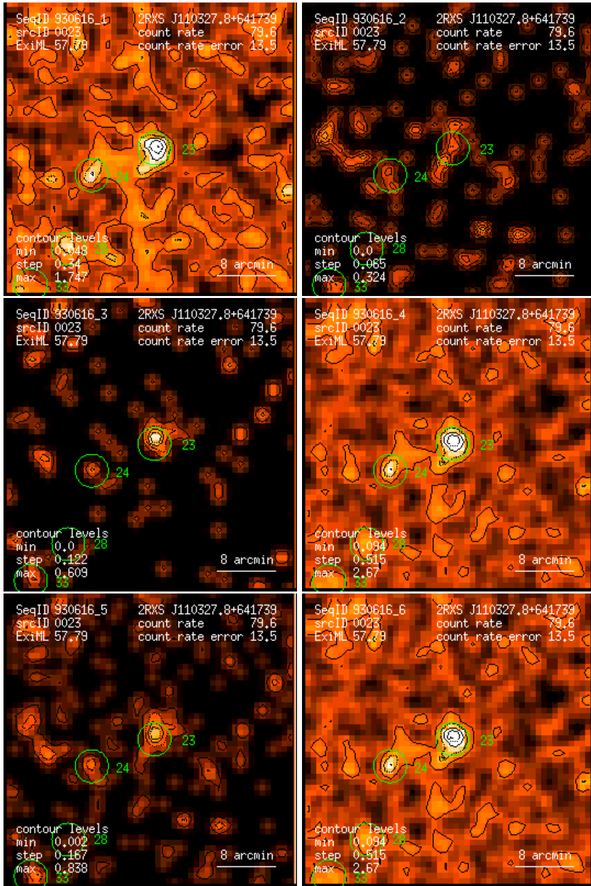
Figure 23: RASS 930616: detection 0023: band rate images, Gaussian filter: (1) PSPC channels 11 – 41, (2) 52 – 90, (3) 91 – 201, (4) 11 – 235, (5) 52 – 201, (6) 11 – 201. Broad band rates in counts/ks. Band rate contour levels in counts/ks/arcmin 2 .
