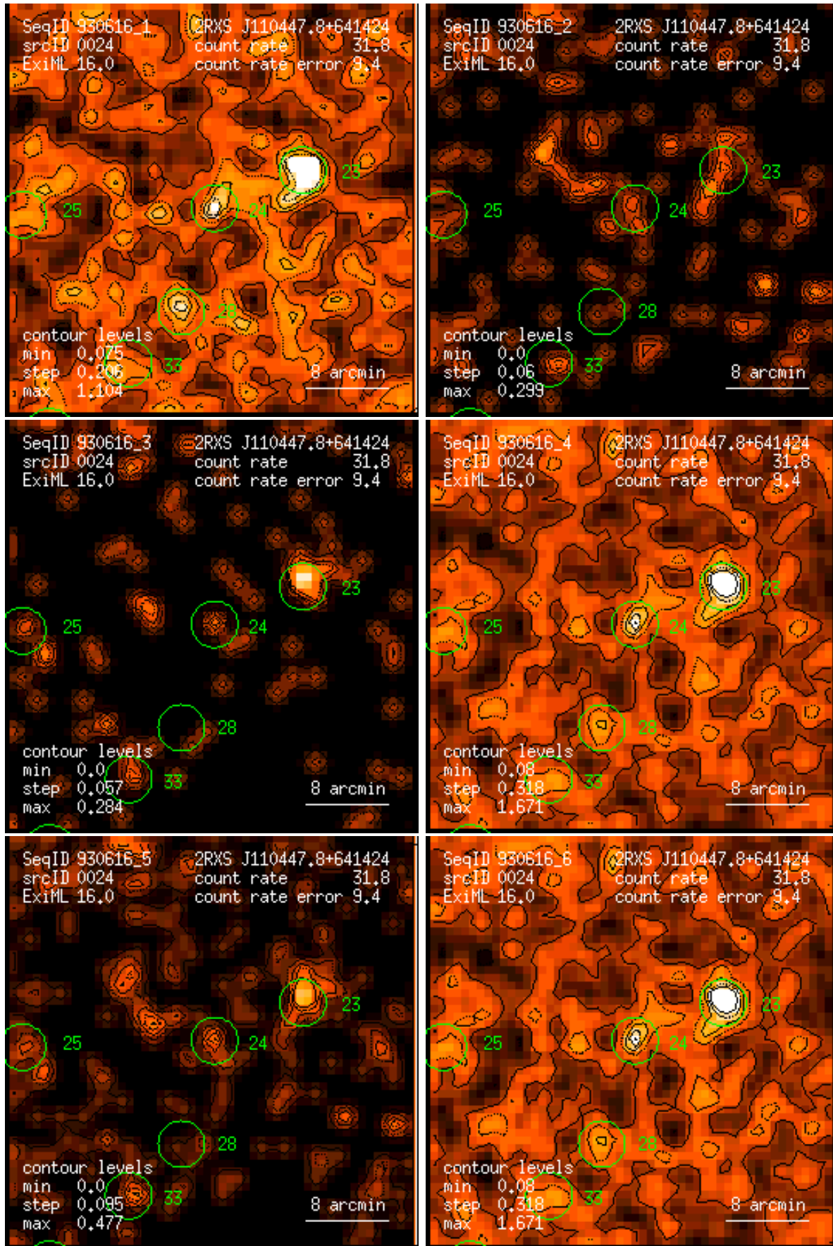
Figure 24: RASS 930616: detection 0024: band rate images, Gaussian filter: (1) PSPC channels 11 – 41, (2) 52 – 90, (3) 91 – 201, (4) 11 – 235, (5) 52 – 201, (6) 11 – 201. Broad band rates in counts/ks. Band rate contour levels in counts/ks/arcmin 2 .
