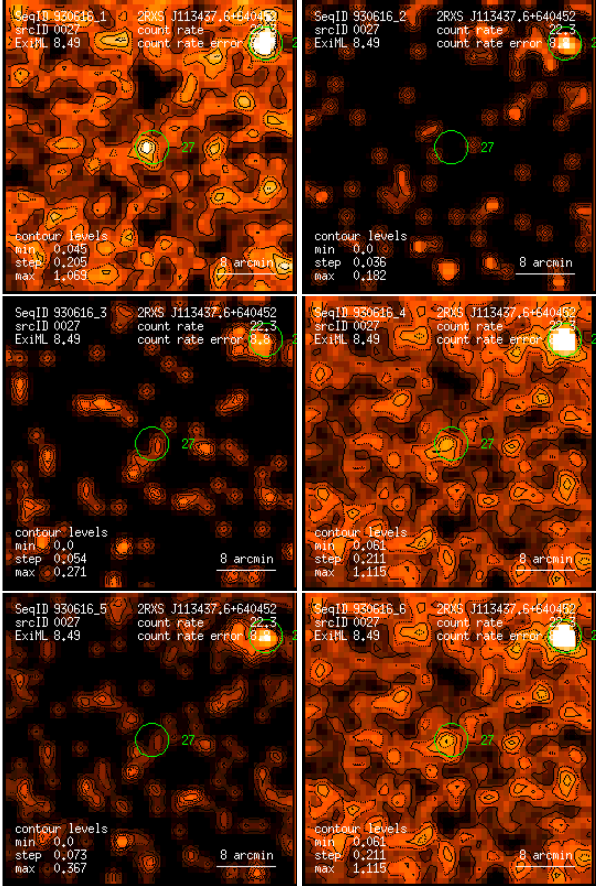
Figure 27: RASS 930616: detection 0027: band rate images, Gaussian filter: (1) PSPC channels 11 – 41, (2) 52 – 90, (3) 91 – 201, (4) 11 – 235, (5) 52 – 201, (6) 11 – 201. Broad band rates in counts/ks. Band rate contour levels in counts/ks/arcmin 2 .
