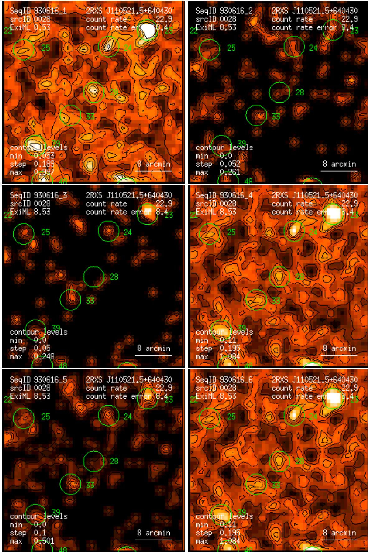
Figure 28: RASS 930616: detection 0028: band rate images, Gaussian filter: (1) PSPC channels 11 – 41, (2) 52 – 90, (3) 91 – 201, (4) 11 – 235, (5) 52 – 201, (6) 11 – 201. Broad band rates in counts/ks. Band rate contour levels in counts/ks/arcmin 2 .
