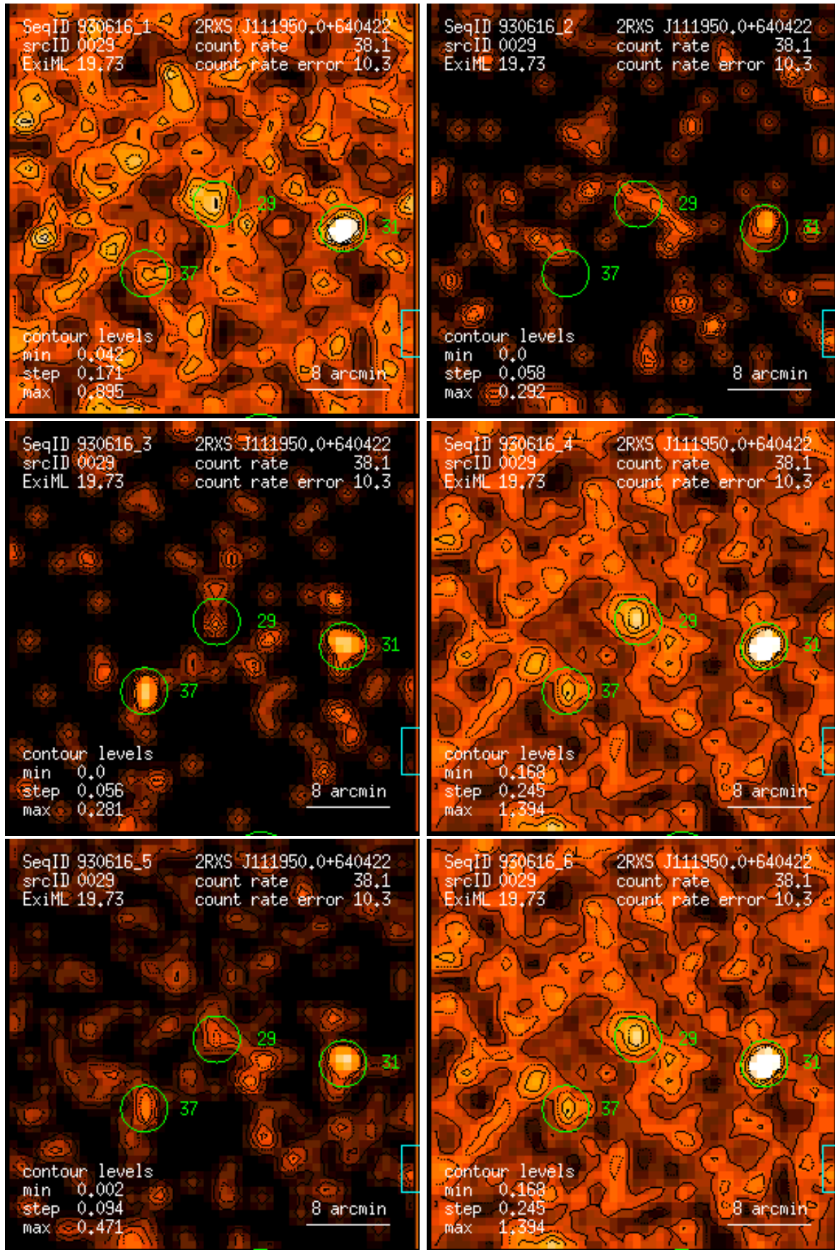
Figure 29: RASS 930616: detection 0029: band rate images, Gaussian filter: (1) PSPC channels 11 – 41, (2) 52 – 90, (3) 91 – 201, (4) 11 – 235, (5) 52 – 201, (6) 11 – 201. Broad band rates in counts/ks. Band rate contour levels in counts/ks/arcmin 2 .
