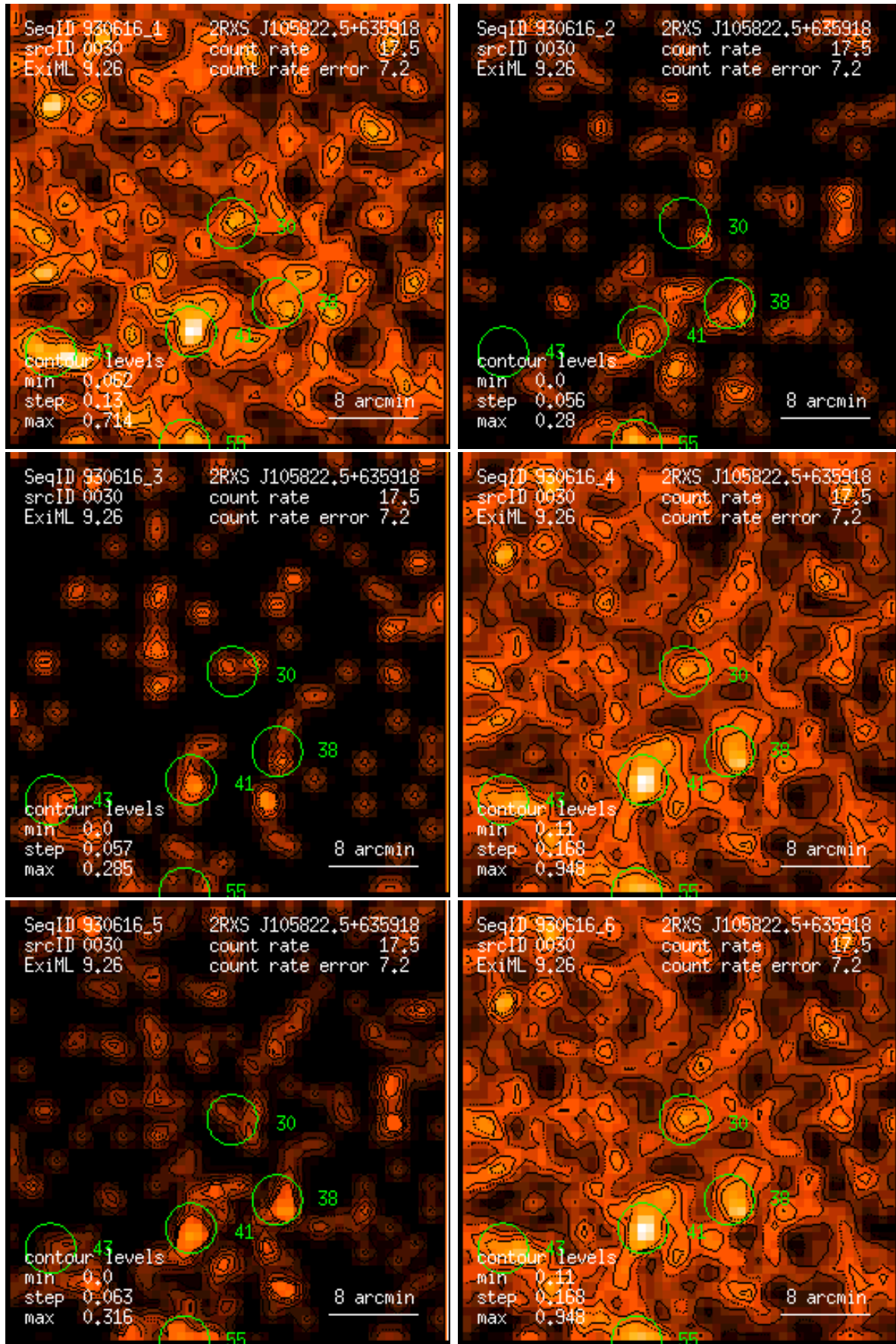
Figure 30: RASS 930616: detection 0030: band rate images, Gaussian filter: (1) PSPC channels 11 – 41, (2) 52 – 90, (3) 91 – 201, (4) 11 – 235, (5) 52 – 201, (6) 11 – 201. Broad band rates in counts/ks. Band rate contour levels in counts/ks/arcmin 2 .
