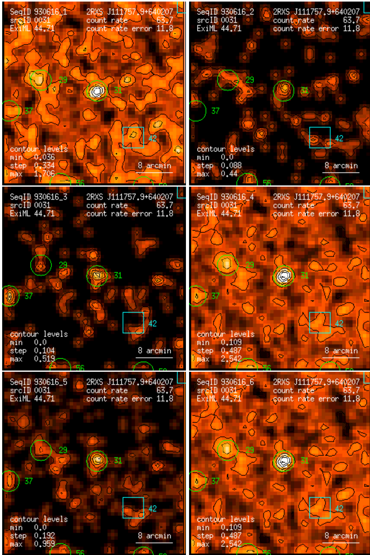
Figure 31: RASS 930616: detection 0031: band rate images, Gaussian filter: (1) PSPC channels 11 – 41, (2) 52 – 90, (3) 91 – 201, (4) 11 – 235, (5) 52 – 201, (6) 11 – 201. Broad band rates in counts/ks. Band rate contour levels in counts/ks/arcmin 2 .
