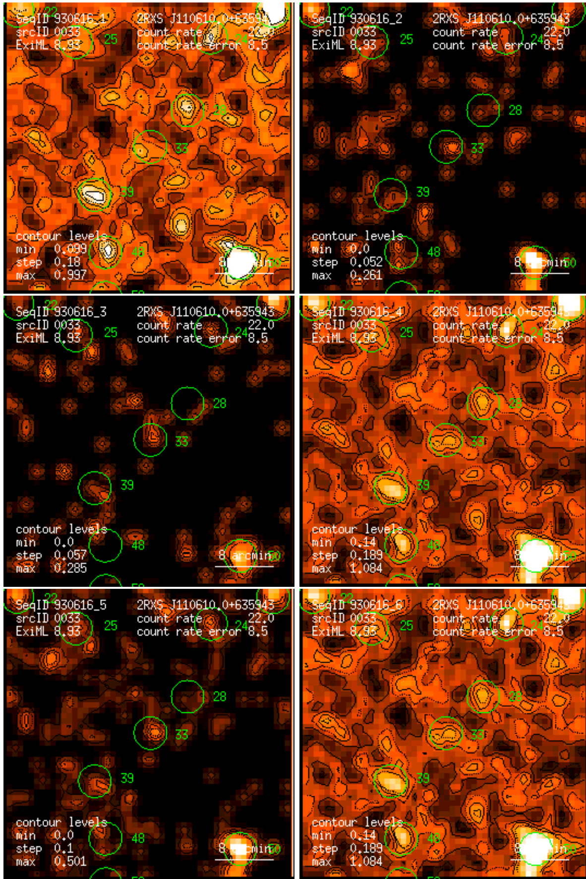
Figure 33: RASS 930616: detection 0033: band rate images, Gaussian filter: (1) PSPC channels 11 – 41, (2) 52 – 90, (3) 91 – 201, (4) 11 – 235, (5) 52 – 201, (6) 11 – 201. Broad band rates in counts/ks. Band rate contour levels in counts/ks/arcmin 2 .
