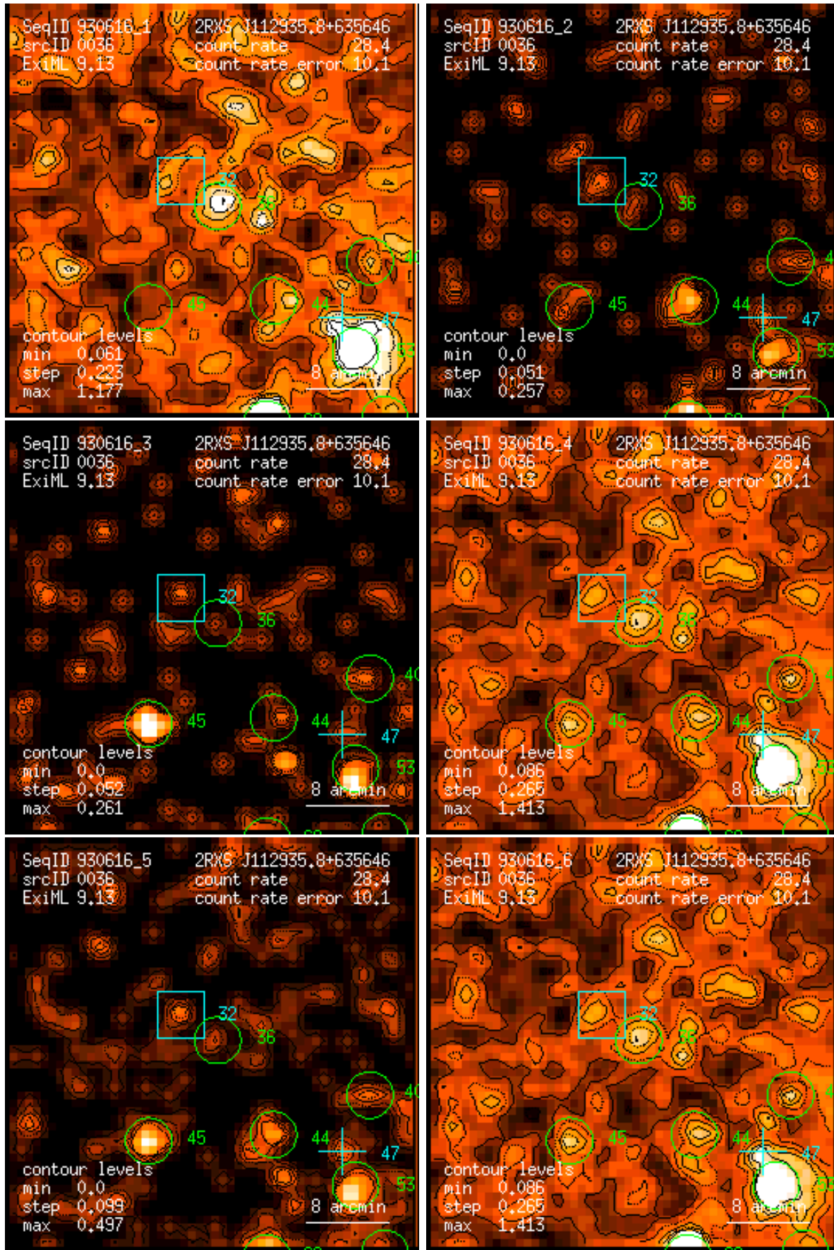
Figure 36: RASS 930616: detection 0036: band rate images, Gaussian filter: (1) PSPC channels 11 – 41, (2) 52 – 90, (3) 91 – 201, (4) 11 – 235, (5) 52 – 201, (6) 11 – 201. Broad band rates in counts/ks. Band rate contour levels in counts/ks/arcmin 2 .
