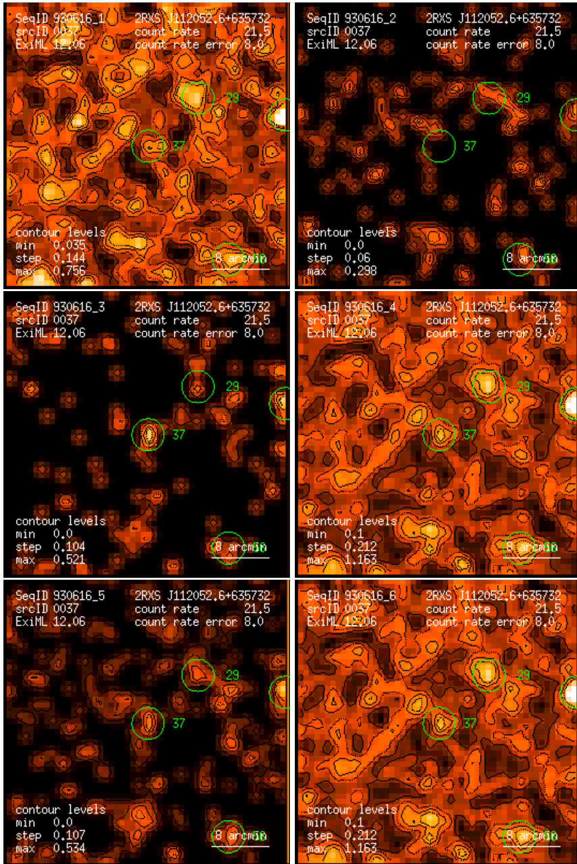
Figure 37: RASS 930616: detection 0037: band rate images, Gaussian filter: (1) PSPC channels 11 – 41, (2) 52 – 90, (3) 91 – 201, (4) 11 – 235, (5) 52 – 201, (6) 11 – 201. Broad band rates in counts/ks. Band rate contour levels in counts/ks/arcmin 2 .
