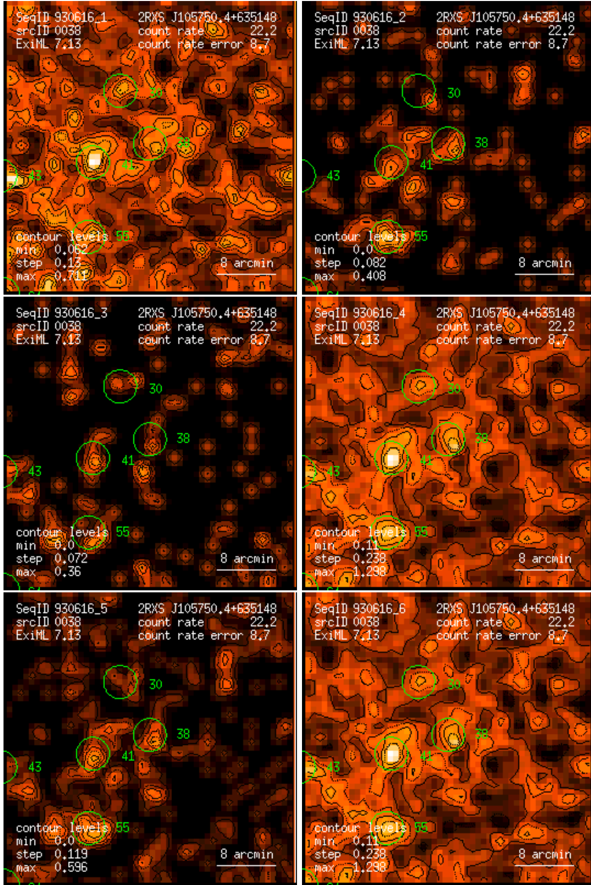
Figure 38: RASS 930616: detection 0038: band rate images, Gaussian filter: (1) PSPC channels 11 – 41, (2) 52 – 90, (3) 91 – 201, (4) 11 – 235, (5) 52 – 201, (6) 11 – 201. Broad band rates in counts/ks. Band rate contour levels in counts/ks/arcmin 2 .
