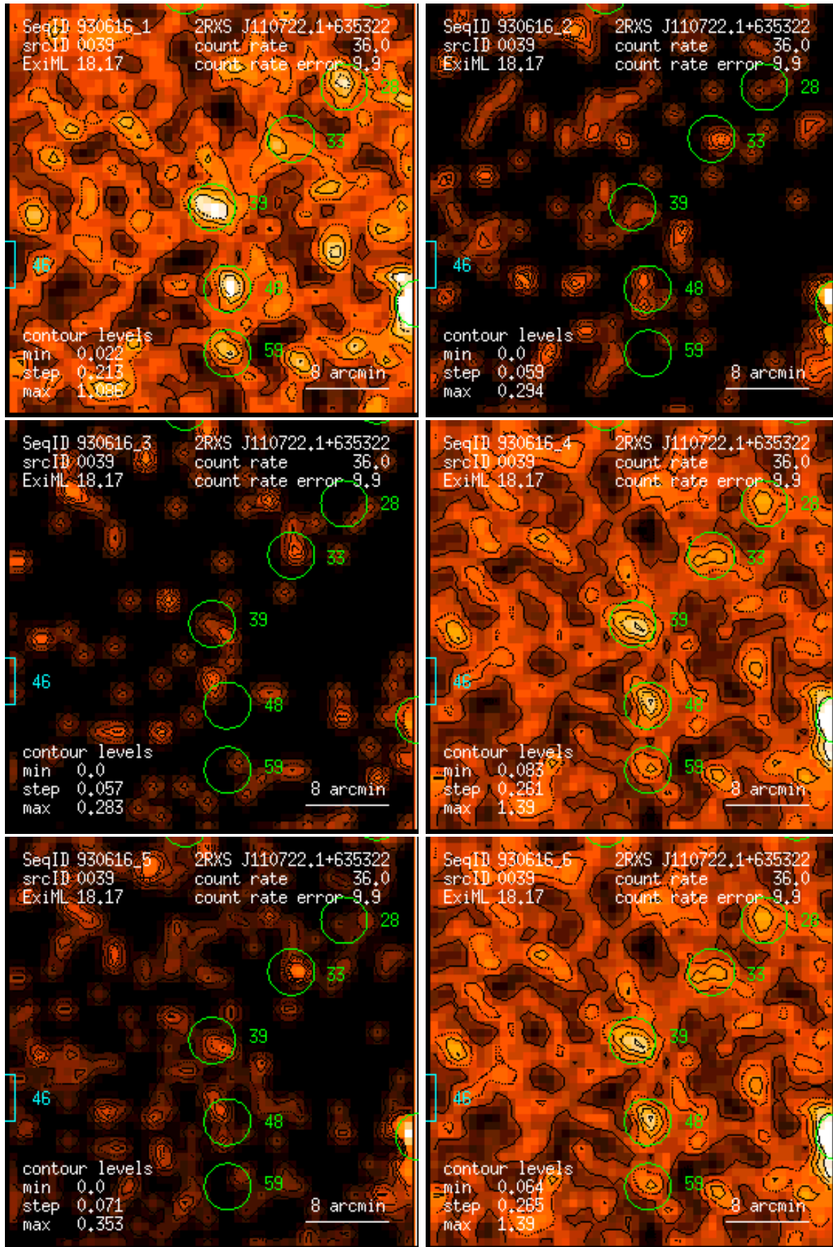
Figure 39: RASS 930616: detection 0039: band rate images, Gaussian filter: (1) PSPC channels 11 – 41, (2) 52 – 90, (3) 91 – 201, (4) 11 – 235, (5) 52 – 201, (6) 11 – 201. Broad band rates in counts/ks. Band rate contour levels in counts/ks/arcmin 2 .
