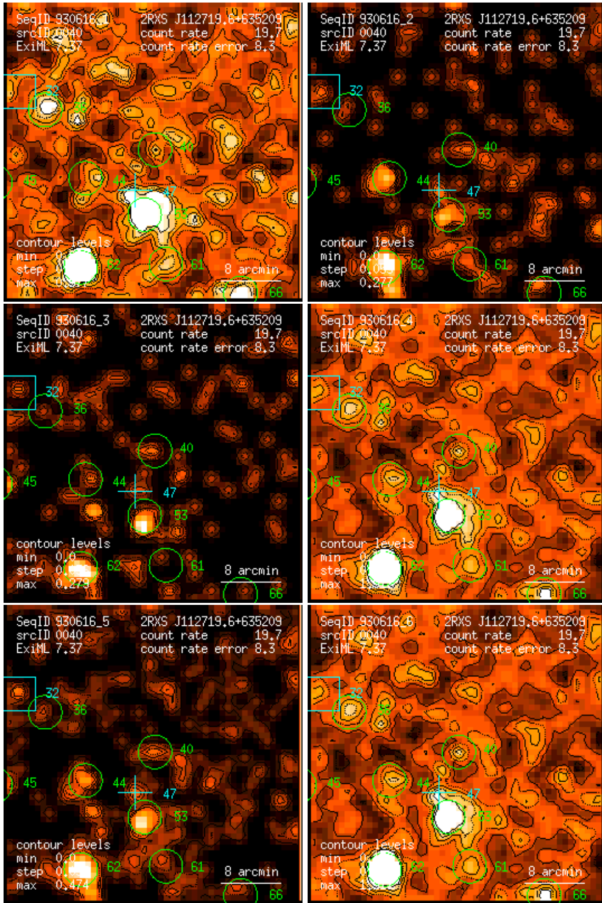
Figure 40: RASS 930616: detection 0040: band rate images, Gaussian filter: (1) PSPC channels 11 – 41, (2) 52 – 90, (3) 91 – 201, (4) 11 – 235, (5) 52 – 201, (6) 11 – 201. Broad band rates in counts/ks. Band rate contour levels in counts/ks/arcmin 2 .
