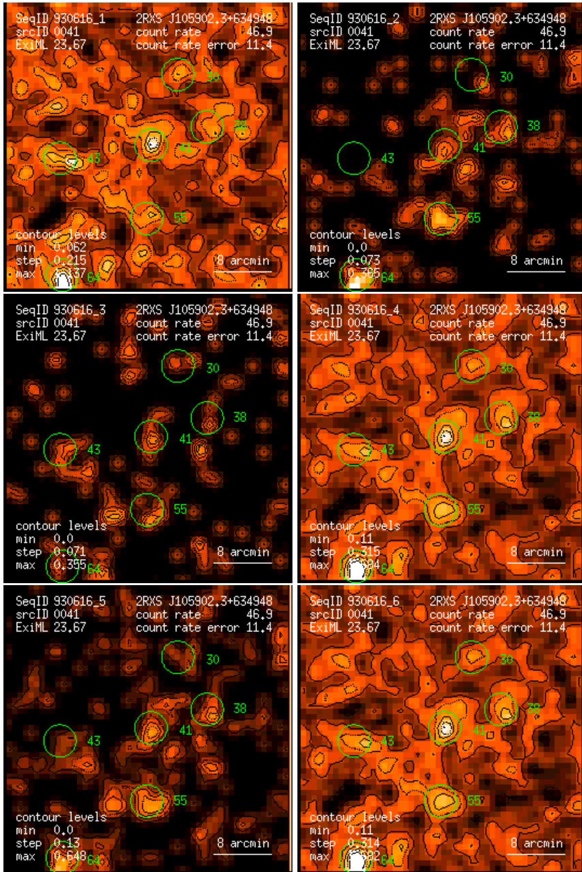
Figure 41: RASS 930616: detection 0041: band rate images, Gaussian filter: (1) PSPC channels 11 – 41, (2) 52 – 90, (3) 91 – 201, (4) 11 – 235, (5) 52 – 201, (6) 11 – 201. Broad band rates in counts/ks. Band rate contour levels in counts/ks/arcmin 2 .
