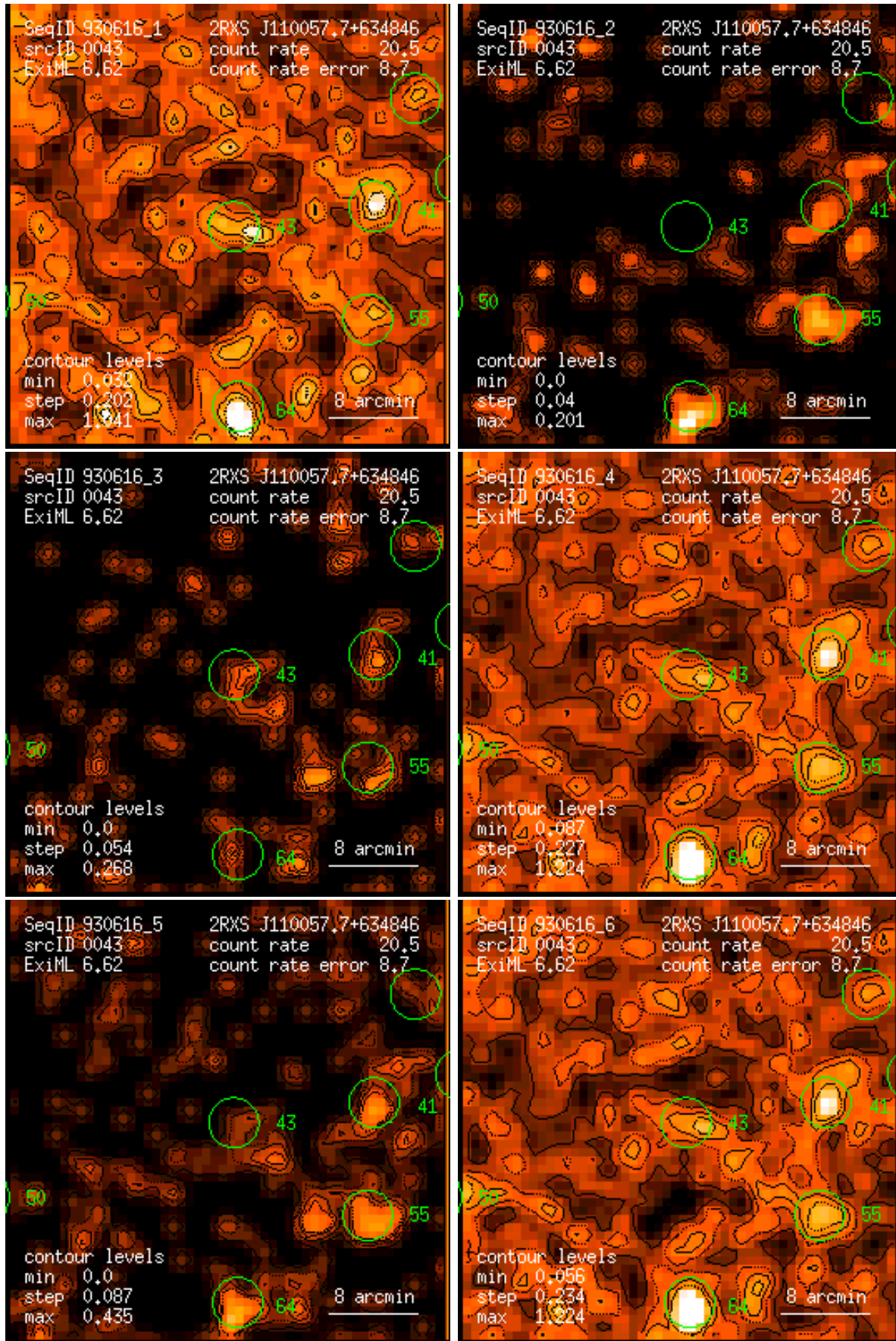
Figure 43: RASS 930616: detection 0043: band rate images, Gaussian filter: (1) PSPC channels 11 – 41, (2) 52 – 90, (3) 91 – 201, (4) 11 – 235, (5) 52 – 201, (6) 11 – 201. Broad band rates in counts/ks. Band rate contour levels in counts/ks/arcmin 2 .
