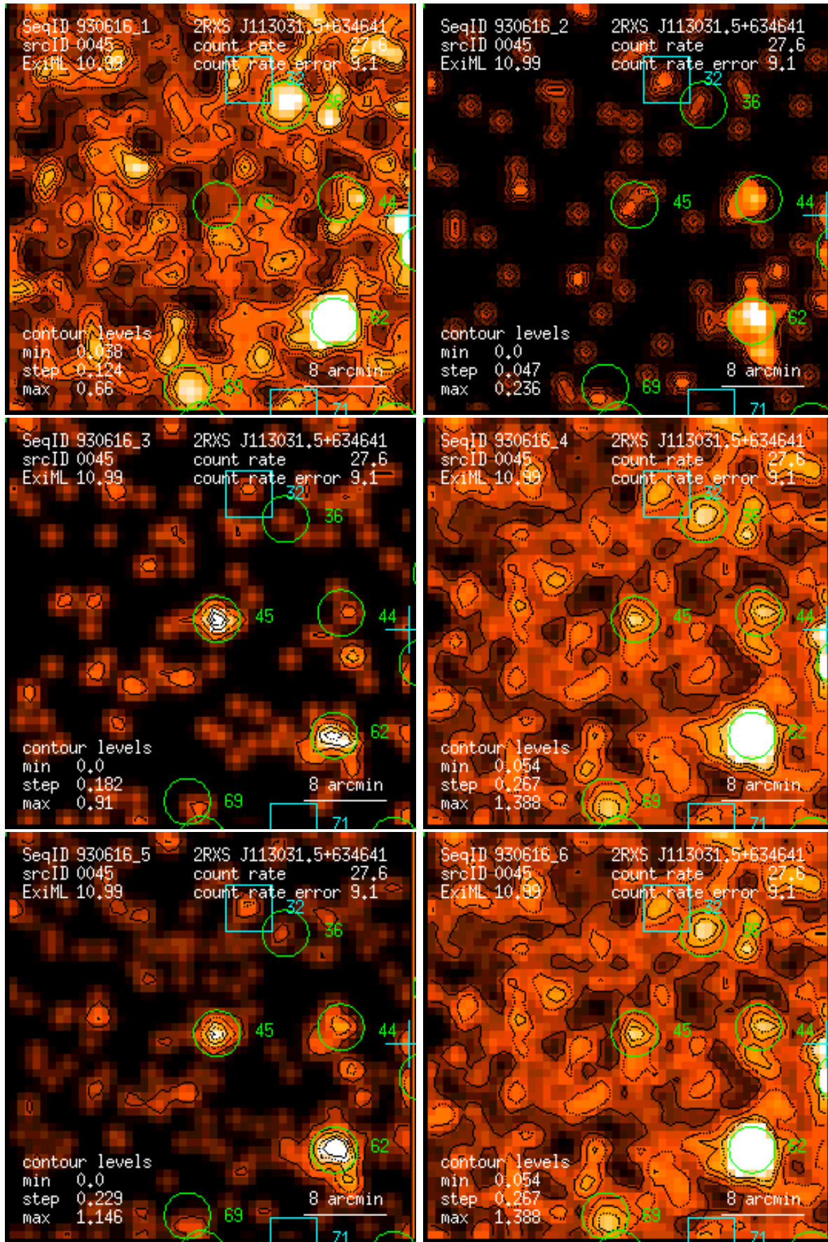
Figure 45: RASS 930616: detection 0045: band rate images, Gaussian filter: (1) PSPC channels 11 – 41, (2) 52 – 90, (3) 91 – 201, (4) 11 – 235, (5) 52 – 201, (6) 11 – 201. Broad band rates in counts/ks. Band rate contour levels in counts/ks/arcmin 2 .
