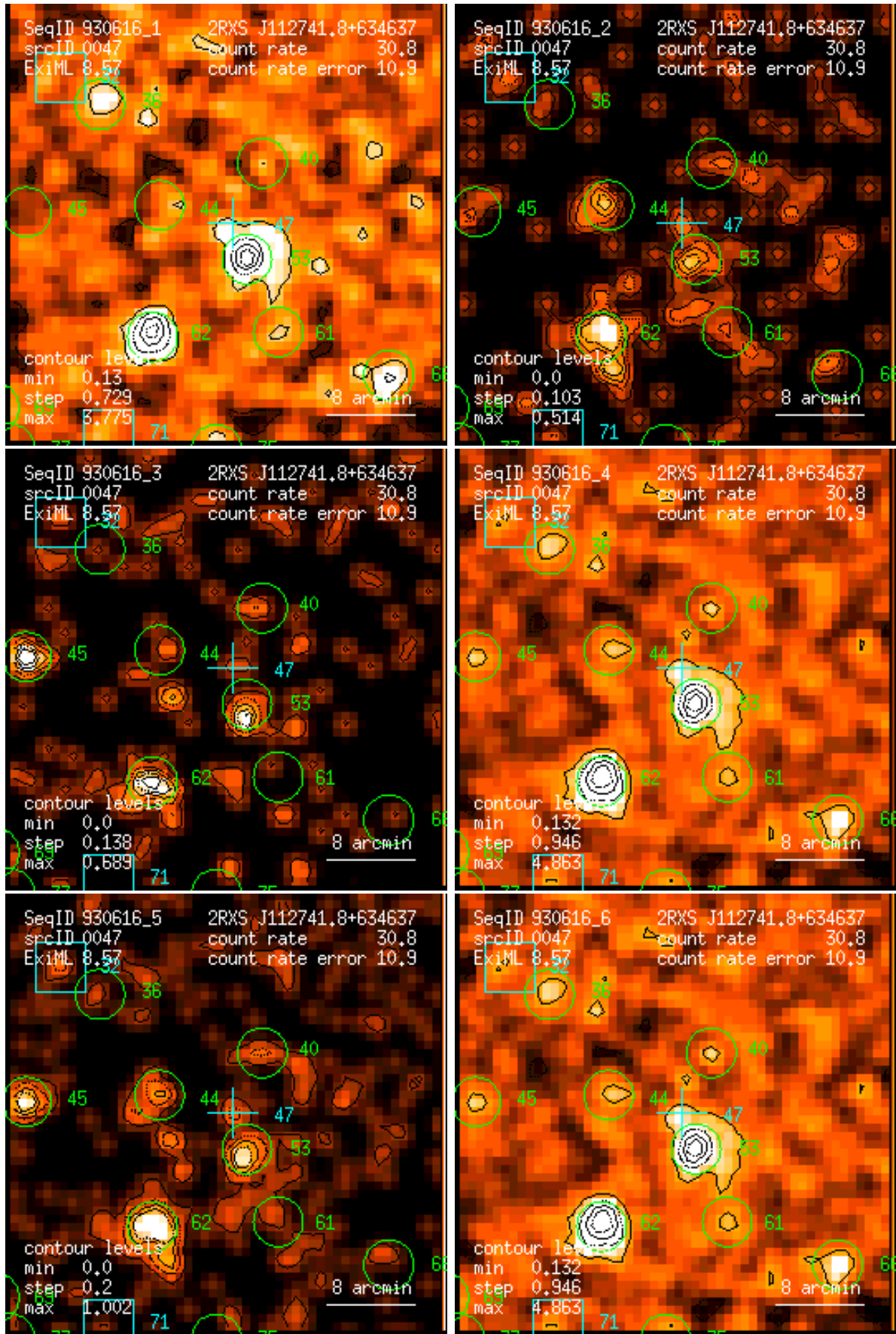
Figure 47: RASS 930616: detection 0047: band rate images, Gaussian filter: (1) PSPC channels 11 – 41, (2) 52 – 90, (3) 91 – 201, (4) 11 – 235, (5) 52 – 201, (6) 11 – 201. Broad band rates in counts/ks. Band rate contour levels in counts/ks/arcmin 2 .
