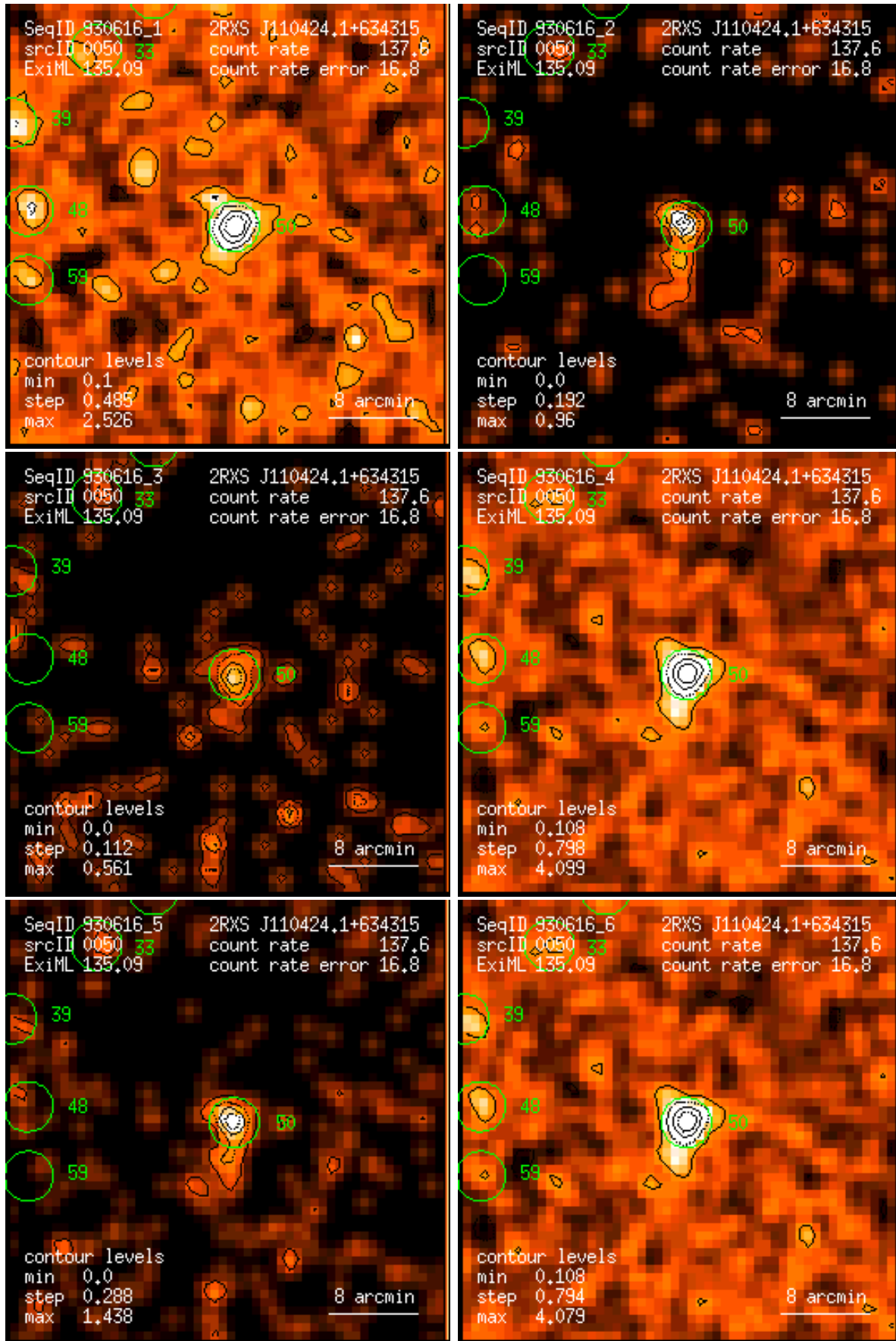
Figure 50: RASS 930616: detection 0050: band rate images, Gaussian filter: (1) PSPC channels 11 – 41, (2) 52 – 90, (3) 91 – 201, (4) 11 – 235, (5) 52 – 201, (6) 11 – 201. Broad band rates in counts/ks. Band rate contour levels in counts/ks/arcmin 2 .
