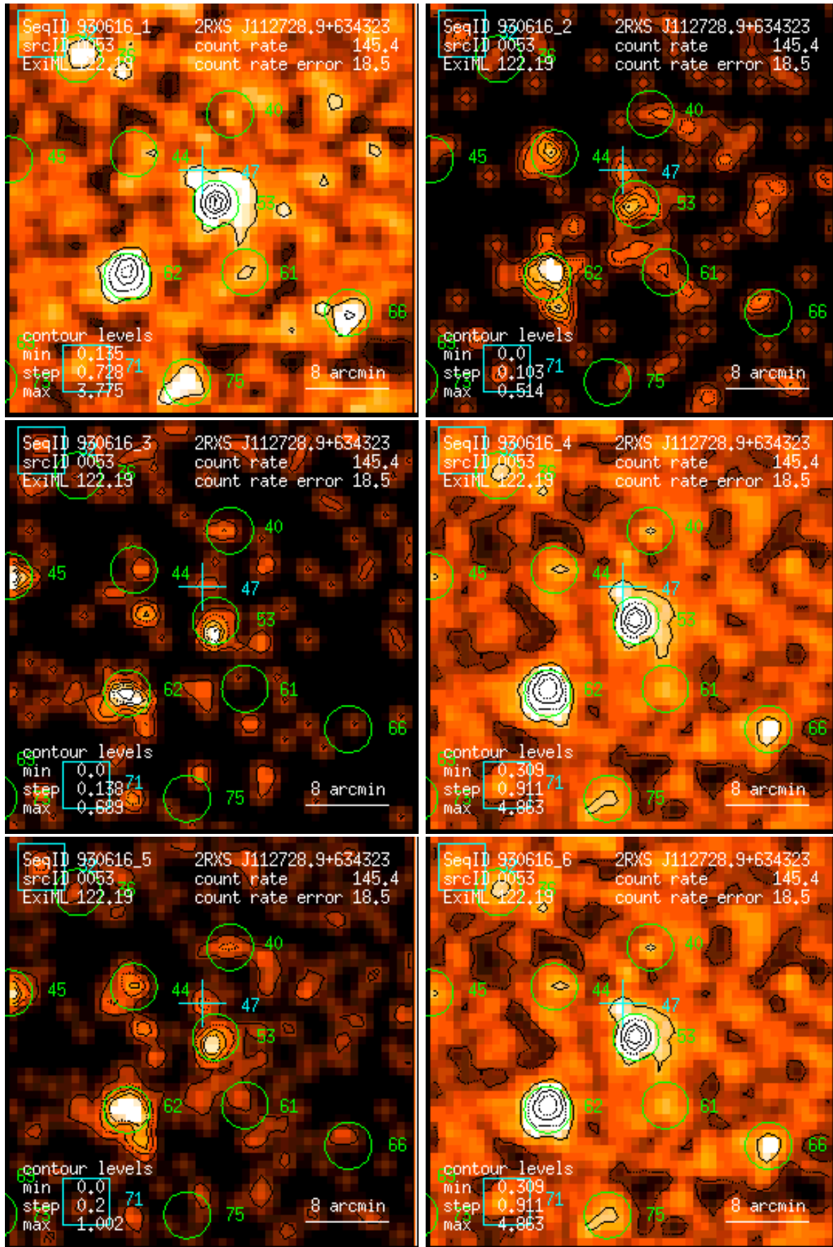
Figure 53: RASS 930616: detection 0053: band rate images, Gaussian filter: (1) PSPC channels 11 – 41, (2) 52 – 90, (3) 91 – 201, (4) 11 – 235, (5) 52 – 201, (6) 11 – 201. Broad band rates in counts/ks. Band rate contour levels in counts/ks/arcmin 2 .
