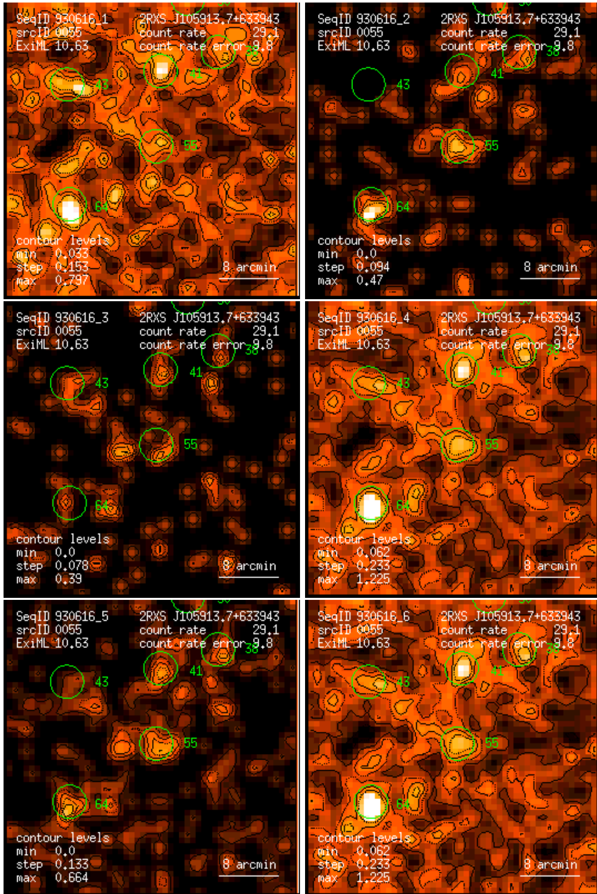
Figure 55: RASS 930616: detection 0055: band rate images, Gaussian filter: (1) PSPC channels 11 – 41, (2) 52 – 90, (3) 91 – 201, (4) 11 – 235, (5) 52 – 201, (6) 11 – 201. Broad band rates in counts/ks. Band rate contour levels in counts/ks/arcmin 2 .
