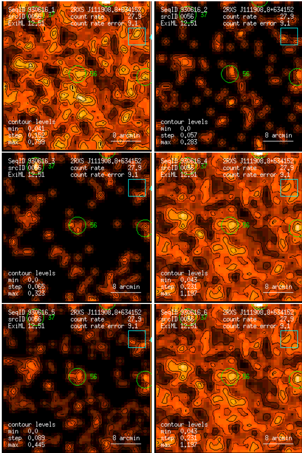
Figure 56: RASS 930616: detection 0056: band rate images, Gaussian filter: (1) PSPC channels 11 – 41, (2) 52 – 90, (3) 91 – 201, (4) 11 – 235, (5) 52 – 201, (6) 11 – 201. Broad band rates in counts/ks. Band rate contour levels in counts/ks/arcmin 2 .
