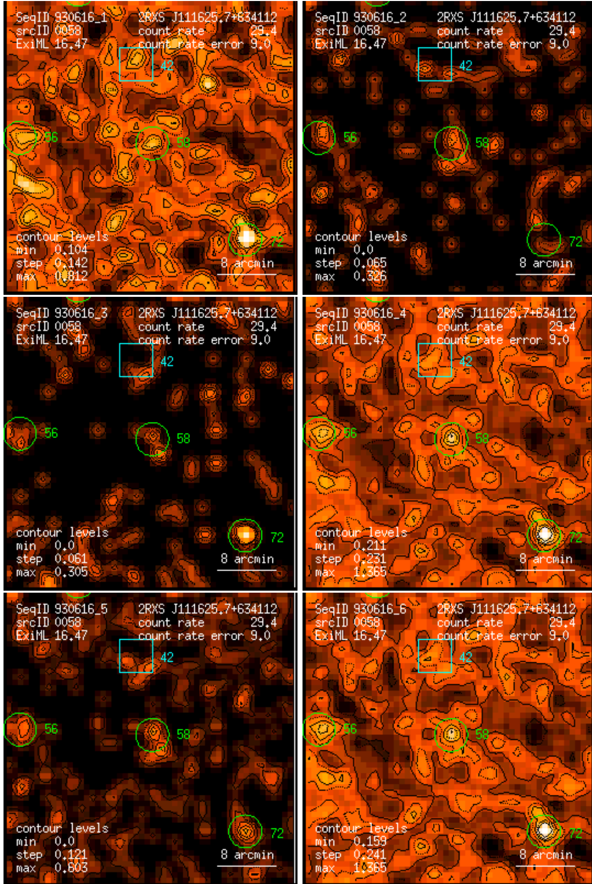
Figure 58: RASS 930616: detection 0058: band rate images, Gaussian filter: (1) PSPC channels 11 – 41, (2) 52 – 90, (3) 91 – 201, (4) 11 – 235, (5) 52 – 201, (6) 11 – 201. Broad band rates in counts/ks. Band rate contour levels in counts/ks/arcmin 2 .
