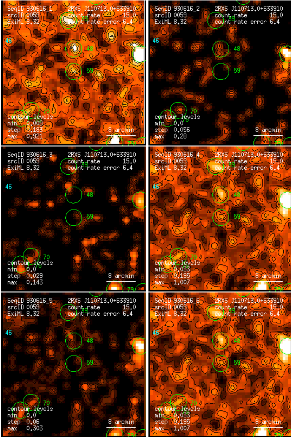
Figure 59: RASS 930616: detection 0059: band rate images, Gaussian filter: (1) PSPC channels 11 – 41, (2) 52 – 90, (3) 91 – 201, (4) 11 – 235, (5) 52 – 201, (6) 11 – 201. Broad band rates in counts/ks. Band rate contour levels in counts/ks/arcmin 2 .
