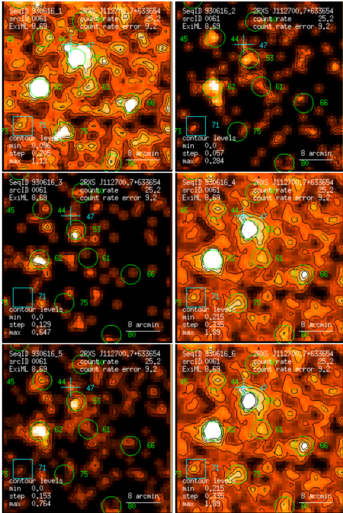
Figure 61: RASS 930616: detection 0061: band rate images, Gaussian filter: (1) PSPC channels 11 – 41, (2) 52 – 90, (3) 91 – 201, (4) 11 – 235, (5) 52 – 201, (6) 11 – 201. Broad band rates in counts/ks. Band rate contour levels in counts/ks/arcmin 2 .
