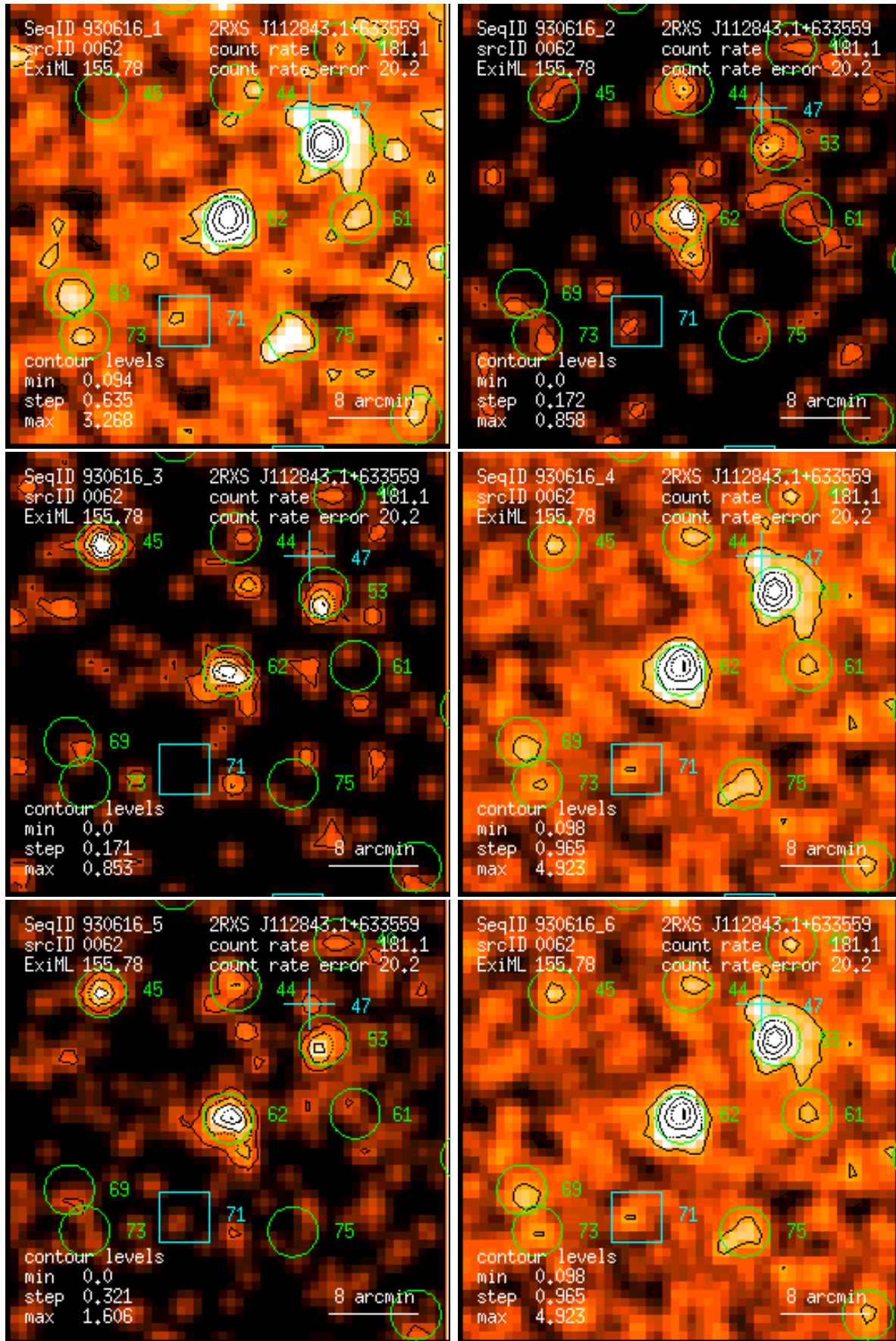
Figure 62: RASS 930616: detection 0062: band rate images, Gaussian filter: (1) PSPC channels 11 – 41, (2) 52 – 90, (3) 91 – 201, (4) 11 – 235, (5) 52 – 201, (6) 11 – 201. Broad band rates in counts/ks. Band rate contour levels in counts/ks/arcmin 2 .
