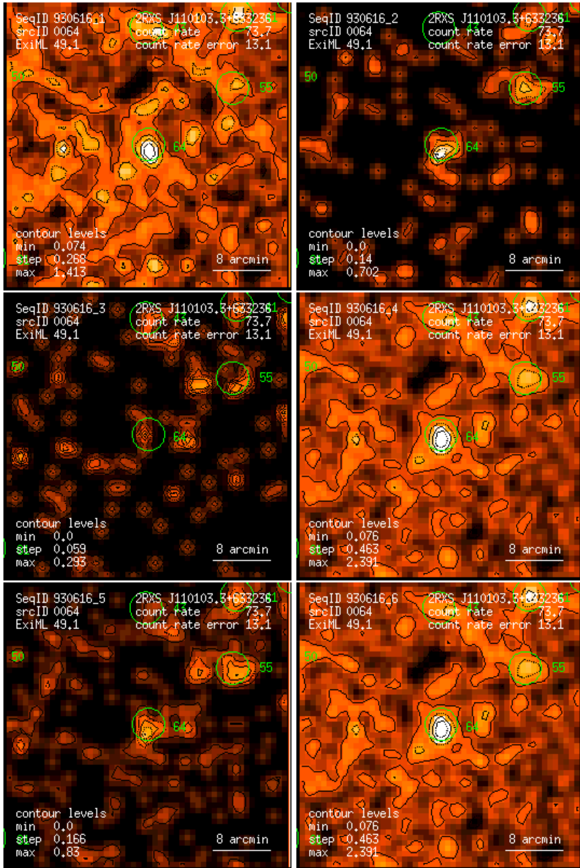
Figure 64: RASS 930616: detection 0064: band rate images, Gaussian filter: (1) PSPC channels 11 – 41, (2) 52 – 90, (3) 91 – 201, (4) 11 – 235, (5) 52 – 201, (6) 11 – 201. Broad band rates in counts/ks. Band rate contour levels in counts/ks/arcmin 2 .
