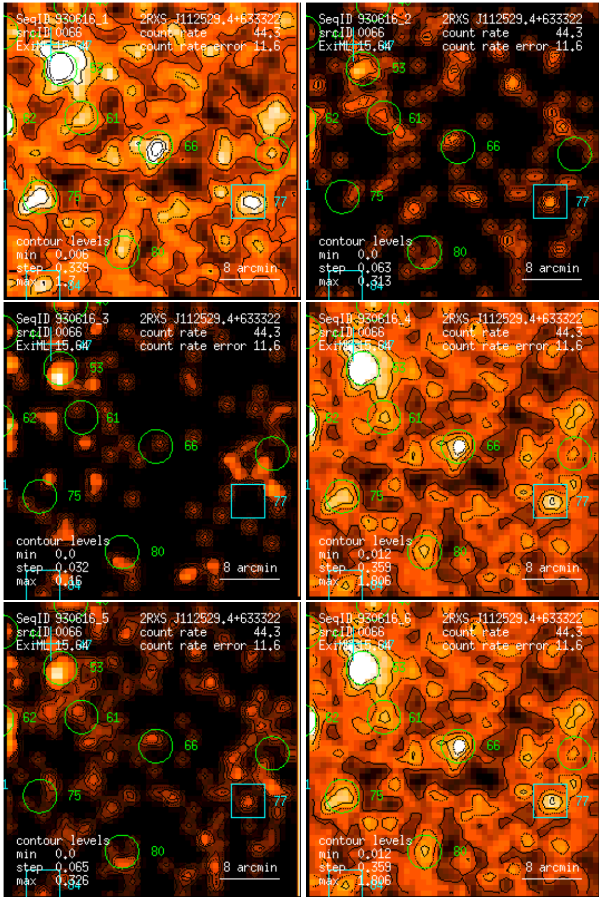
Figure 66: RASS 930616: detection 0066: band rate images, Gaussian filter: (1) PSPC channels 11 – 41, (2) 52 – 90, (3) 91 – 201, (4) 11 – 235, (5) 52 – 201, (6) 11 – 201. Broad band rates in counts/ks. Band rate contour levels in counts/ks/arcmin 2 .
