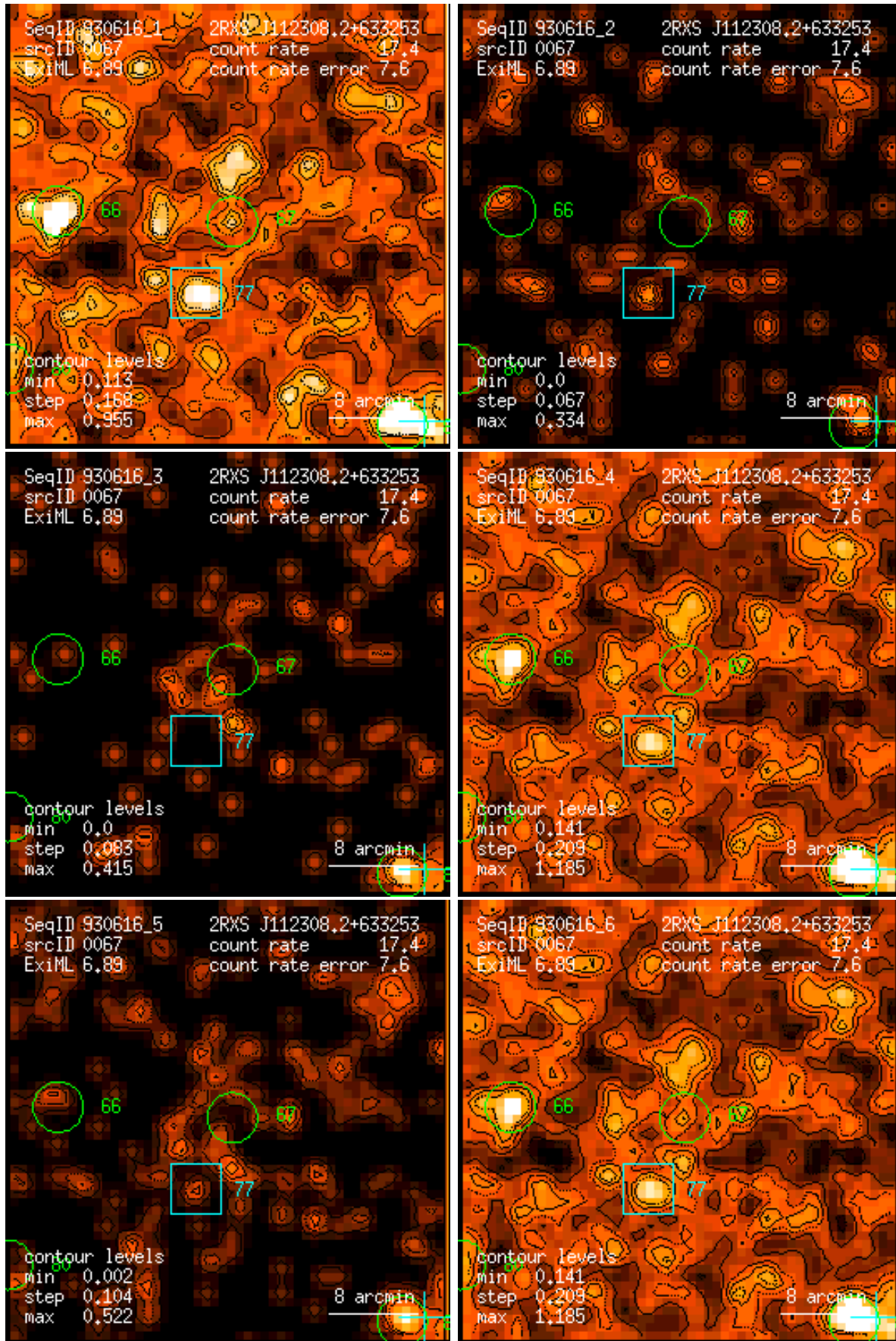
Figure 67: RASS 930616: detection 0067: band rate images, Gaussian filter: (1) PSPC channels 11 – 41, (2) 52 – 90, (3) 91 – 201, (4) 11 – 235, (5) 52 – 201, (6) 11 – 201. Broad band rates in counts/ks. Band rate contour levels in counts/ks/arcmin 2 .
