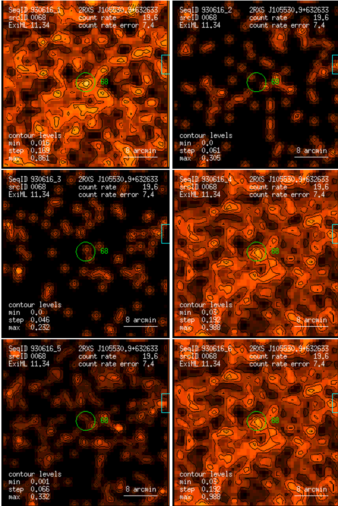
Figure 68: RASS 930616: detection 0068: band rate images, Gaussian filter: (1) PSPC channels 11 – 41, (2) 52 – 90, (3) 91 – 201, (4) 11 – 235, (5) 52 – 201, (6) 11 – 201. Broad band rates in counts/ks. Band rate contour levels in counts/ks/arcmin 2 .
