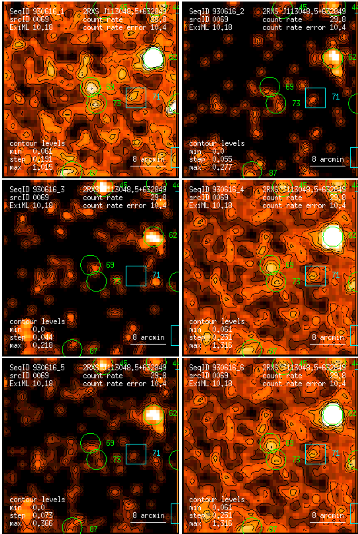
Figure 69: RASS 930616: detection 0069: band rate images, Gaussian filter: (1) PSPC channels 11 – 41, (2) 52 – 90, (3) 91 – 201, (4) 11 – 235, (5) 52 – 201, (6) 11 – 201. Broad band rates in counts/ks. Band rate contour levels in counts/ks/arcmin 2 .
