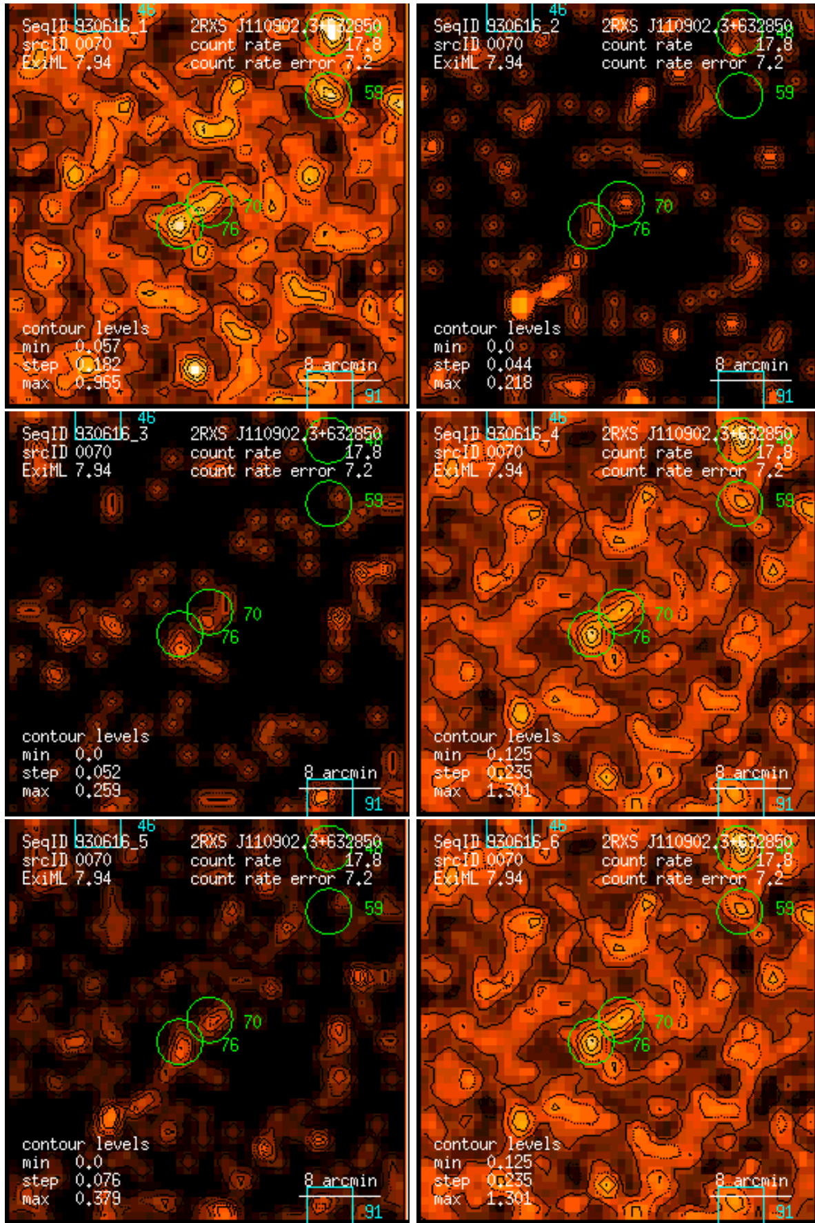
Figure 70: RASS 930616: detection 0070: band rate images, Gaussian filter: (1) PSPC channels 11 – 41, (2) 52 – 90, (3) 91 – 201, (4) 11 – 235, (5) 52 – 201, (6) 11 – 201. Broad band rates in counts/ks. Band rate contour levels in counts/ks/arcmin 2 .
