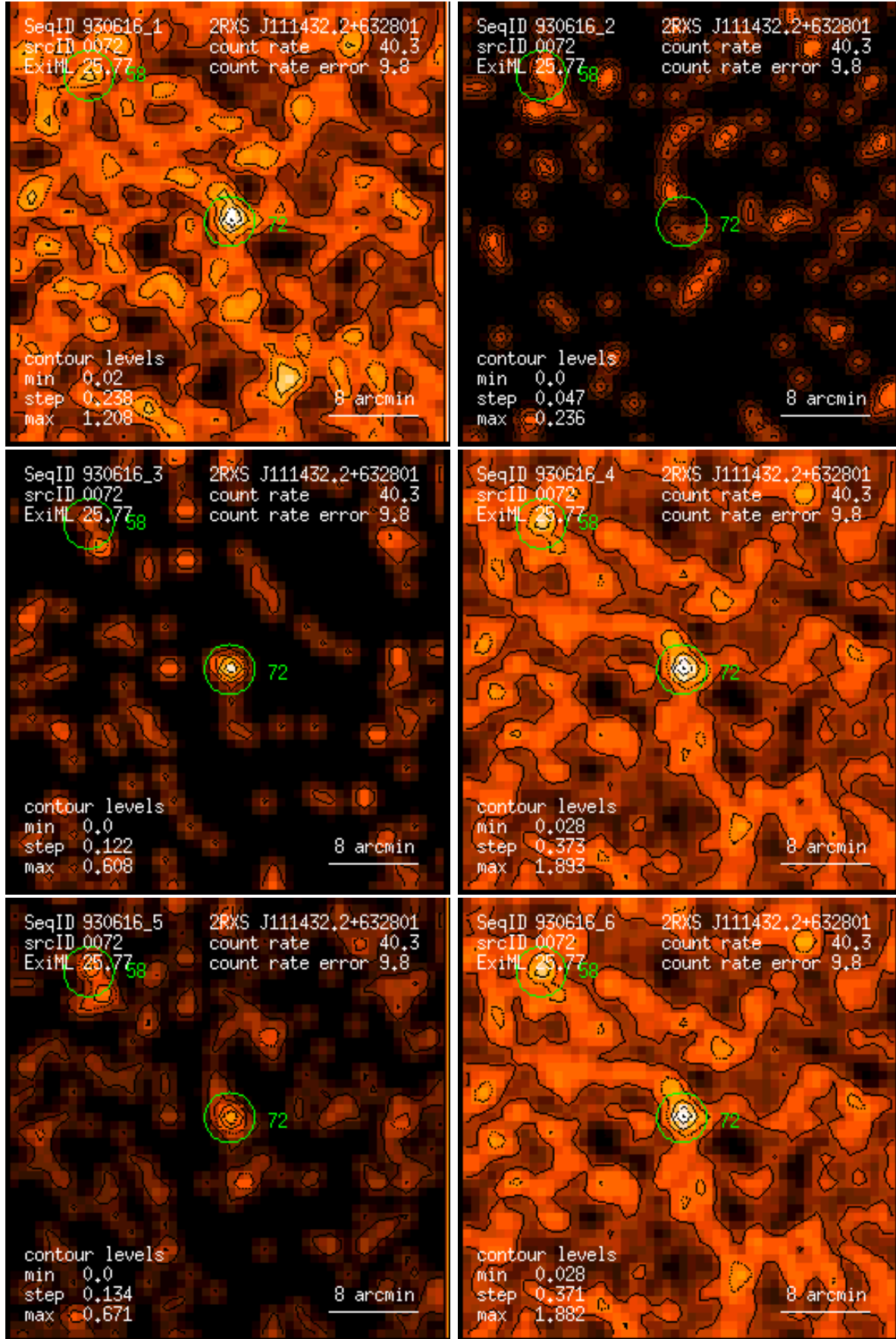
Figure 72: RASS 930616: detection 0072: band rate images, Gaussian filter: (1) PSPC channels 11 – 41, (2) 52 – 90, (3) 91 – 201, (4) 11 – 235, (5) 52 – 201, (6) 11 – 201. Broad band rates in counts/ks. Band rate contour levels in counts/ks/arcmin 2 .
