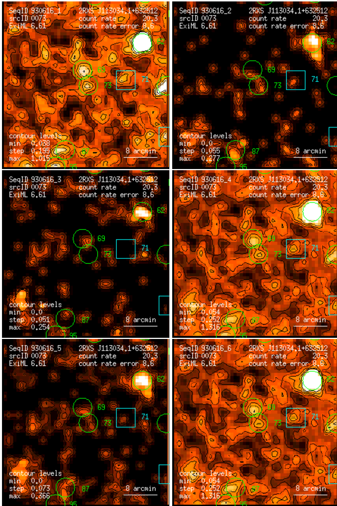
Figure 73: RASS 930616: detection 0073: band rate images, Gaussian filter: (1) PSPC channels 11 – 41, (2) 52 – 90, (3) 91 – 201, (4) 11 – 235, (5) 52 – 201, (6) 11 – 201. Broad band rates in counts/ks. Band rate contour levels in counts/ks/arcmin 2 .
