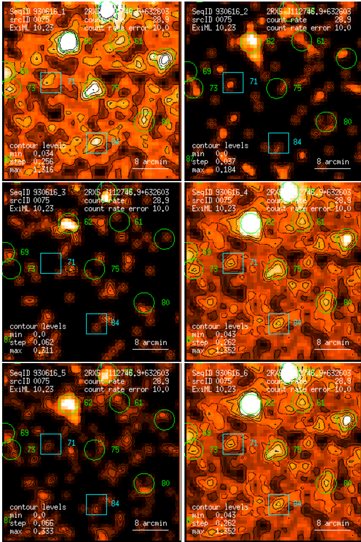
Figure 75: RASS 930616: detection 0075: band rate images, Gaussian filter: (1) PSPC channels 11 – 41, (2) 52 – 90, (3) 91 – 201, (4) 11 – 235, (5) 52 – 201, (6) 11 – 201. Broad band rates in counts/ks. Band rate contour levels in counts/ks/arcmin 2 .
