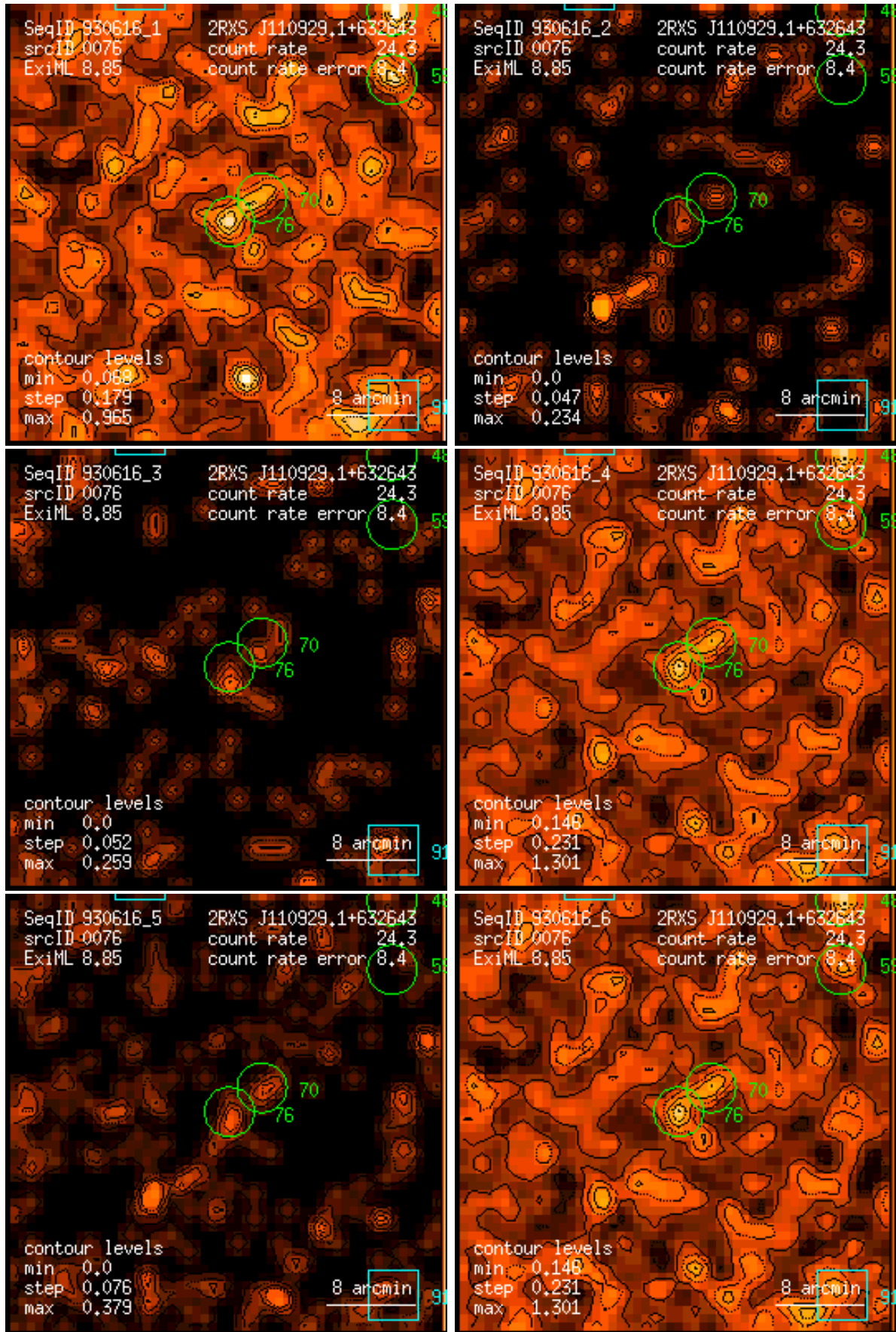
Figure 76: RASS 930616: detection 0076: band rate images, Gaussian filter: (1) PSPC channels 11 – 41, (2) 52 – 90, (3) 91 – 201, (4) 11 – 235, (5) 52 – 201, (6) 11 – 201. Broad band rates in counts/ks. Band rate contour levels in counts/ks/arcmin 2 .
